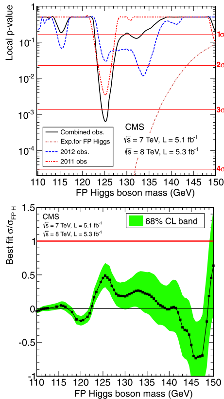
Fig. 7. (Top) The observed local p -value p_0 as a function of the FP Higgs boson mass in the range 110–150 GeV. The dashed-dotted line shows the expected local p -values should a fermiophobic Higgs boson with a mass m_H exist. The contributions to the expected limit for each run period are shown. (Bottom) The best-fit \hat{\mu} = \sigma/\sigma_{\text{FPH}} as a function of the FP Higgs boson mass in the range 110–150 GeV. The band corresponds to the \pm 1 standard deviation uncertainty on the \hat{\mu} values.
