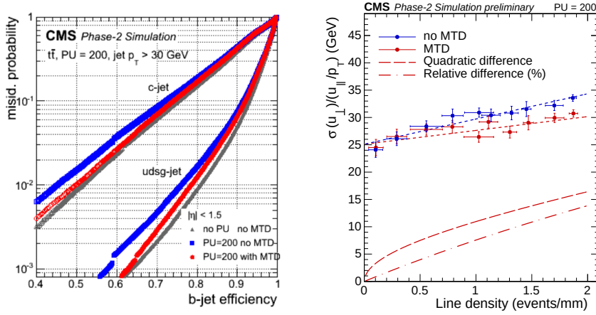
Figure 4: B-tagging efficiency as a function of the misidentification probability for the b-tagging algorithms with and without the MTD (left) and resolution of the transverse missing momentum with and without the MTD (right).
