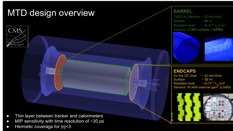
Figure 2: Diagram showing the MTD design with details about the technologies being used in both the BTL and ETL.
