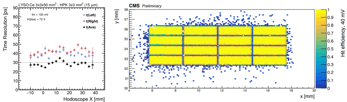
Figure 3: Time resolution as a function of the longitudinal coordinate of the crystal (left) and hit efficiency for an array of 4x4 LGAD pixels (right).
