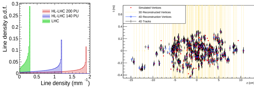
Figure 1: Distribution of the density of vertices per unit length (left) and expected distribution of vertices in the z-t plane at the HL-LHC.
