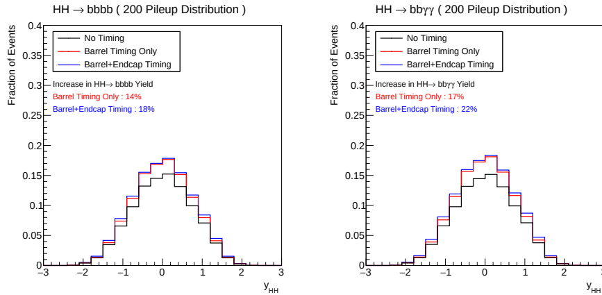
Figure 5: Yields as a function of the Higgs rapidity for the HH \rightarrow bbbb (left) and HH \rightarrow bb\gamma\gamma final states (right).
