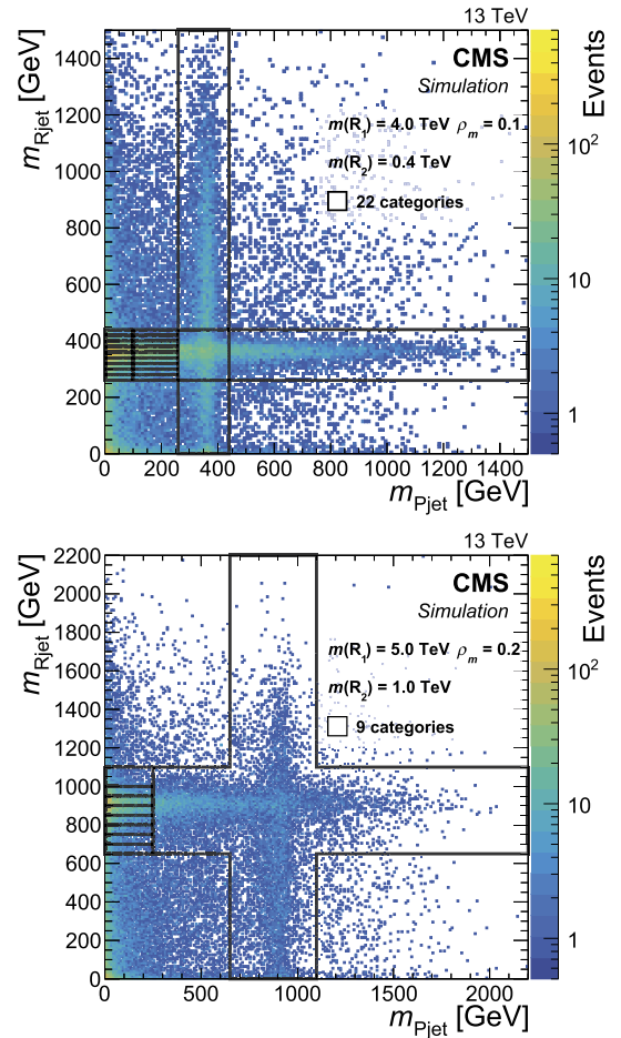
Fig. 2. In the simulation, the reconstructed mass of the R_2 jet candidate ( m_{R\text{jet}} ) vs. the reconstructed mass of the P_3 jet candidate ( m_{P\text{jet}} ) for R_1 resonance events originating from two different mass hypotheses. The upper plot is for a G_{KK} with a mass m(G_{KK}) = m(R_1) = 4 TeV, decaying to a radion with a mass m(\phi) = m(R_2) = 0.4 TeV and a gluon. The 22 event categories in this plane, within which the search in the dijet mass distribution is conducted, are shown with black boxes. The lower plot is for the same decay sequence, with masses m(G_{KK}) = 5 TeV and m(\phi) = 1 TeV, for which the number of event categories is 9. For both plots, the cross-like shape is approximately centered on the second resonance pole mass m(R_2) for both the horizontal and the vertical axes.
