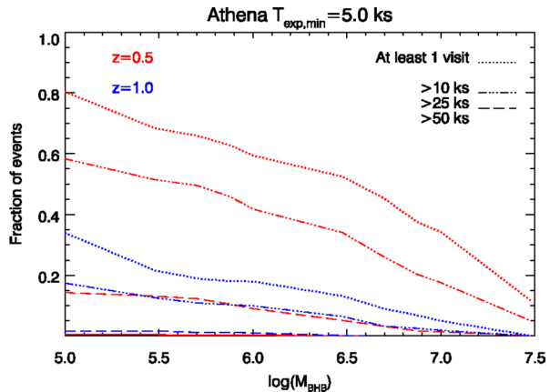
Fig. 13 Fraction of LISA events observed by the Athena /WFI FoV at least once prior to the merging time as a function of the event total BH mass ( dotted lines ). Different colors represent different SMBH binary redshifts ( red : z \sim 0.5 ; blue : z \sim 1 ). Different dashed line styles represent the total accumulated exposure time prior to merging, according to the legend in the inset . The minimum exposure time of each pointing is assumed to be 5 ks
