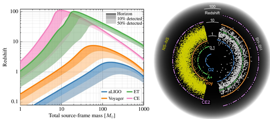
Fig. 5 Left : Detection horizons and 10% and 50% response distances for four GW detectors, LIGO A+ (aLIGO in the figure), LIGO Voyager, ET, and CE, as a function of the binary’s mass, for equal-mass binaries. Figure available from [17] and appears in [18]. Right : Populations of binary NSs (left half) and binary BHs (right half) for binaries that follow the Madau-Dickinson star-formation rate with a characteristic delay time of 100 Myr. Also shown are the detection horizons of different GW detectors. The figure is available from [19]
