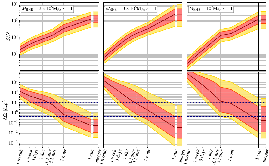
Fig. 11 Signal-to-noise ratio ( S/N ) (top) and sky localization error \Delta\Omega in \text{deg}^2 (bottom) versus time to merger for precessing binaries with total mass equal to 3 \times 10^5 M_\odot (left panel), 3 \times 10^6 M_\odot (central panel), 10^7 M_\odot (right panel) as computed in [88]. The sources are located at z = 1 . The binary mass ratio of these sources is extracted randomly between [0.1-1] , the spin between [0-1] and polarization, inclination and sky position angles are extracted from a sphere. Full precessing inspiral with higher harmonics waveforms are used to carry out the analysis up to one hour before coalescing. The signal is extrapolated down to merger using a simplified waveform and scaling the uncertainty on \Delta\Omega with (S/N)^{-2} . Shaded areas are the 68% and 95% confidence interval computed over 10^4 systems and the dark solid line is the median value. The horizontal dashed line denotes the Field of View (FoV) ( \sim 0.4 \text{ deg}^2 ) of the WFI on-board Athena . The 10 \text{ deg}^2 wider FoV of LSST is denoted with a dotted line. It is noticeable that at merger a large fraction of the sources is in the Athena /WFI FoV.
