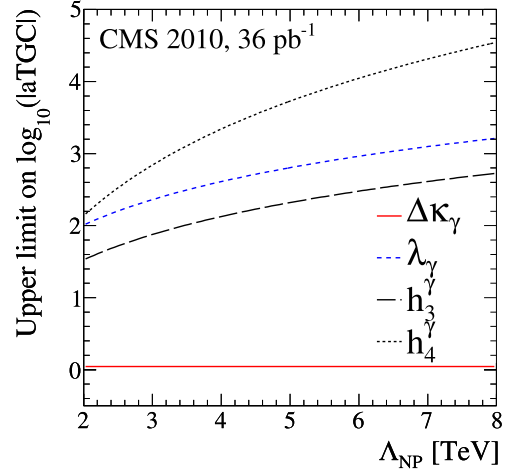
Fig. 7. Upper 95% CL limits on \log_{10}(|\text{aTGC}|) as a function of \Lambda_{\text{NP}} for \Delta\kappa_\gamma , \lambda_\gamma , h_3^\gamma , and h_4^\gamma . Limits on the latter two couplings are similar to those for h_3^Z and h_4^Z . These limits refer to the formulation in which the new physics Lagrangian terms are scaled with \alpha/\Lambda_{\text{NP}}^n , where \Lambda_{\text{NP}} is the characteristic energy scale of new physics and \alpha is the aTGC.
