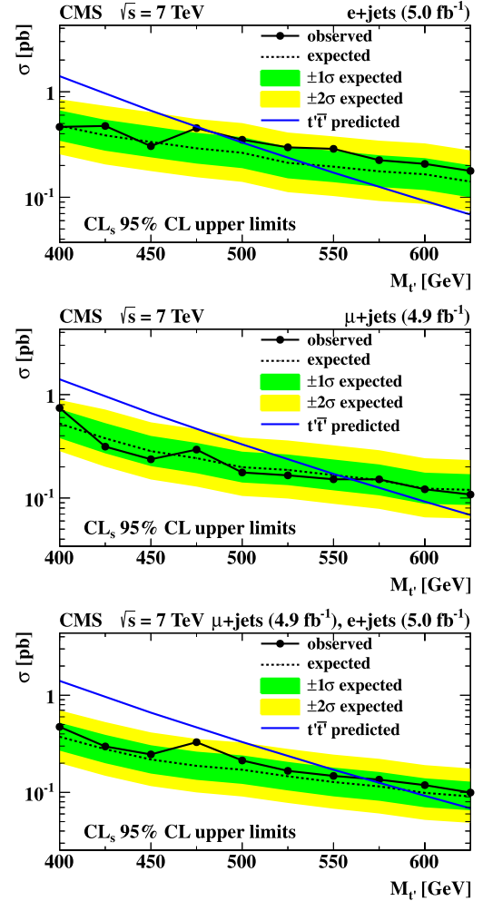
Fig. 6. The observed (solid line with points) and expected (dotted line) 95% CL upper limits on the t'\bar{t}' production cross section as a function of the t' -quark mass for e + \text{jets} (top), \mu + \text{jets} (middle), and combined (bottom) channels. The \pm 1 and \pm 2 standard deviation ranges for the expected limits are shown by the bands. The theoretical t'\bar{t}' cross section is shown by the continuous line without points.
