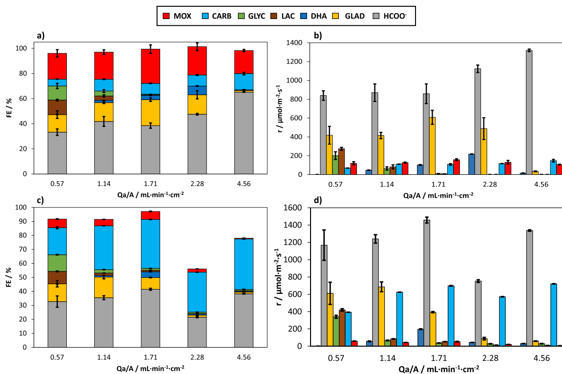
Fig. 7. a) Faradaic Efficiencies (FE) and b) production rates (r) of the glycerol oxidation products quantified as a function of the anolyte flow rate per geometric anode surface area (Qa/A) at current densities (j) of 45 mA·cm -2 ; c) Faradaic Efficiencies (FE) and d) production rates (r) of the glycerol oxidation products quantified as a function of the anolyte flow rate per geometric anode surface area (Qa/A) at current densities (j) of 90 mA·cm -2 .
