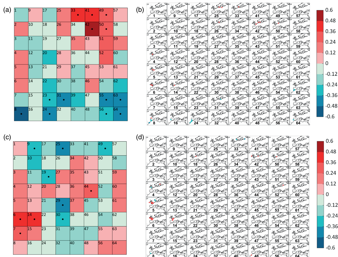
FIGURE 11 (a) Correlation between weather type (WT) occurrence and NAO winter index (significant marked with a dot); (b) correlation between the occurrence of coastal compound events and NAO winter index (only significant shown) along European coastlines; (c, d) same for WEPA index, for the European WT classification (Figure 3) [Colour figure can be viewed at wileyonlinelibrary.com ]
