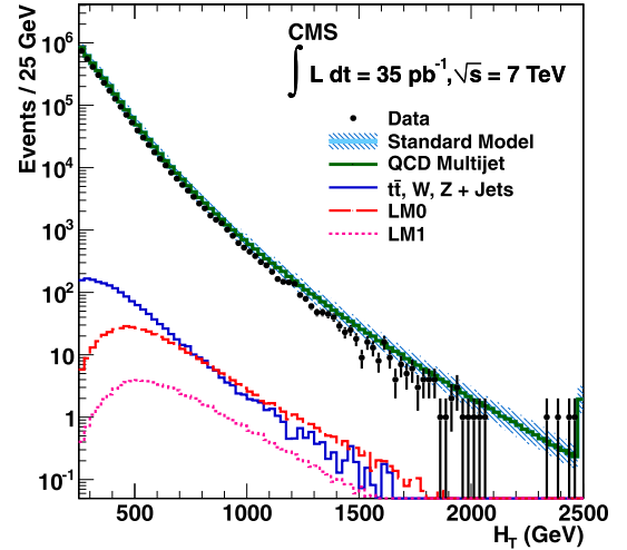
Fig. 1. H_T distribution after preselection, for data as well as for all standard model backgrounds and two SUSY signal samples with parameter sets LM0 and LM1, normalized to an integrated luminosity of 35 \text{ pb}^{-1} . The hatched area corresponds to the uncertainty in the SM estimate as defined in Section 3.1. The SM distributions are only displayed for illustration purposes, as they are the result of Monte Carlo simulation, while the actual estimate of the background from SM processes in this search is based on data, as described in detail in Section 4.
