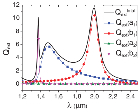
Fig. 1 Extinction cross section Q_{\text{ext}} versus the wavelength \lambda for a 240 nm Ge sphere (the refraction index m_p = 4 is constant and real in this wavelength range). The contribution of each term in the Mie expansion is also shown. The red line corresponds to the magnetic dipole contribution.
