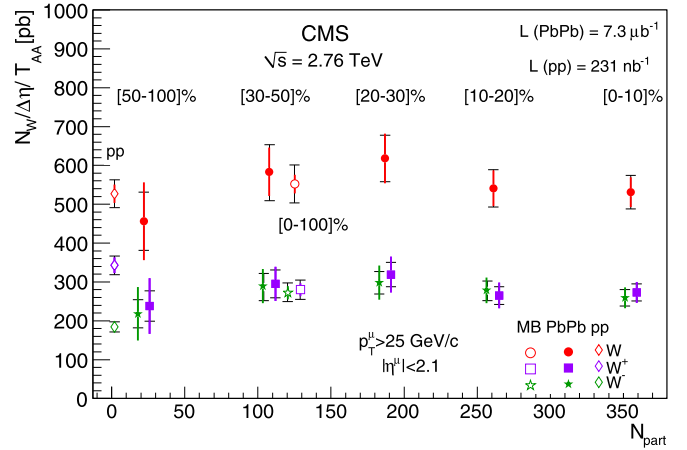
Fig. 2. Centrality dependence of normalised W \rightarrow \mu\nu_\mu cross sections ( (1/T_{AA})(N_W/\Delta\eta) ) in PbPb collisions, for all W candidates (red-filled points) and, separated by charge, W^+ (violet-filled squares) and W^- (green-filled stars). The open symbols at N_{\text{part}} \approx 120 represent the MB events. At N_{\text{part}} = 2 , the corresponding cross sections are displayed for pp collisions divided by \Delta\eta , for the same \sqrt{s} . For clarity, both W^+ and W^- points are slightly shifted on the horizontal axis. The cross sections are given for the phase space region |\eta^\mu| < 2.1 and p_T^\mu > 25 GeV/c. The error bars represent the statistical, and the horizontal lines the systematic, uncertainties. (For interpretation of the references to colour in this figure legend, the reader is referred to the web version of this Letter.)
