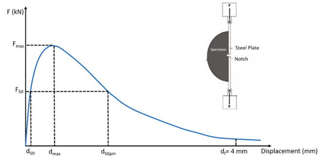
Fig. 5. Stress-displacement curve and Fénix test set-up.
