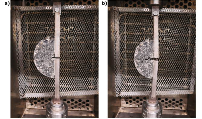
Fig. 6. Fénix test configuration and specimen a) before and b) after the test.
