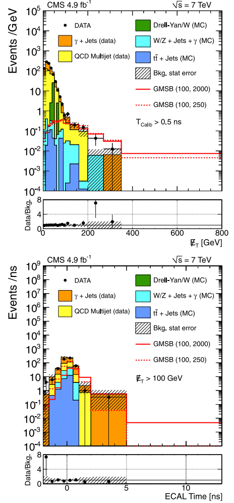
Fig. 6. The one-dimensional projection after all selection requirements for \cancel{E}_T for events with T_{\text{calib}} > 0.5 ns (top) and for ECAL timing (bottom) for events with \cancel{E}_T > 100 GeV. The multijet and \gamma + jets backgrounds are normalized to the yields from the fit. The rest of the backgrounds are fixed according to the integrated luminosity of the data. The GMSB (100, 2000) benchmark point corresponds to \Lambda = 100 TeV, c\tau = 2000 mm and the GMSB (100, 250) benchmark point corresponds to \Lambda = 100 TeV, c\tau = 250 mm. (For interpretation of the references to color in this figure legend, the reader is referred to the web version of this Letter.)
