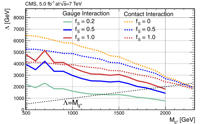
Fig. 4. Contours of excluded parameters for the gauge and contact interaction q^* production mechanisms. For a given f_s assumption, each (M_{q^*}, \Lambda) below the limit curve is excluded. The bump in the \Lambda contour at M_{q^*} = 700 GeV for the gauge interaction production models is a direct consequence of the downward fluctuation on the upper limit on the cross section observed at M_{q^*} = 700 GeV (Fig. 3).
