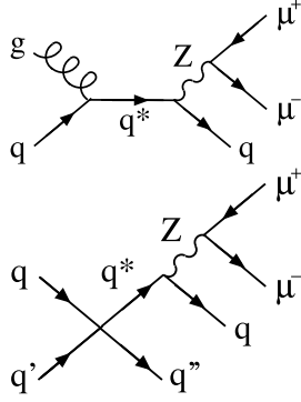
Fig. 1. Feynman diagrams for the production of q^* \rightarrow qZ , Z \rightarrow \mu^+\mu^- via (top) a gauge interaction and (bottom) a contact interaction. Charge conjugation of an initial state quark is implied in both diagrams. Permutation of the quark isospin is implied for the contact interaction diagram.
