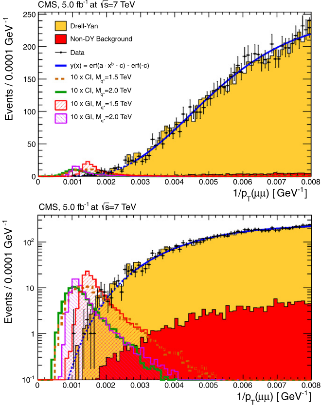
Fig. 2. Distributions of 1/p_T(\mu\mu) for data (points with error bars), simulated SM backgrounds (stacked histograms), and simulated signal models (overlaid histograms). Top: linear scale. Bottom: logarithmic scale. The signal models use either gauge interaction (GI) or contact interaction (CI) simulated with the assumptions of f = f' = f_s = 1 and M_{q^*} = \Lambda . The blue solid line corresponds to the analytical template fit in the region defined by 1/p_T(\mu\mu) \in [0.0028, 0.008] \text{ GeV}^{-1} . The contribution labeled “Non-DY Background” represents the sum over all the other sources of prompt backgrounds, t\bar{t} , Z \rightarrow \tau^+\tau^- , diboson, and non-prompt backgrounds, jets misidentified as muons through multijet and W plus jets final states. The total number of SM background events is rescaled to the number of events observed in data, using the relative background contributions as obtained from simulation. The normalization of the signal distributions is increased by a factor ten. (For interpretation of the references to color in this figure legend, the reader is referred to the web version of this or Letter.)
