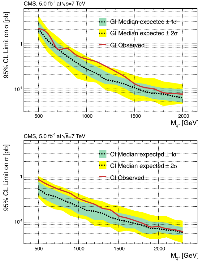
Fig. 3. Observed and expected 95% CL upper limits on the cross section of q^* \rightarrow qZ for the benchmark models derived with the CL_s limit setting criterion: (top) gauge interaction production, (bottom) contact interaction production. The results shown are obtained assuming all new couplings equal to the SM couplings between ordinary fermions ( f = f' = f_s = 1 ) and \Lambda = M_{q^*} .
