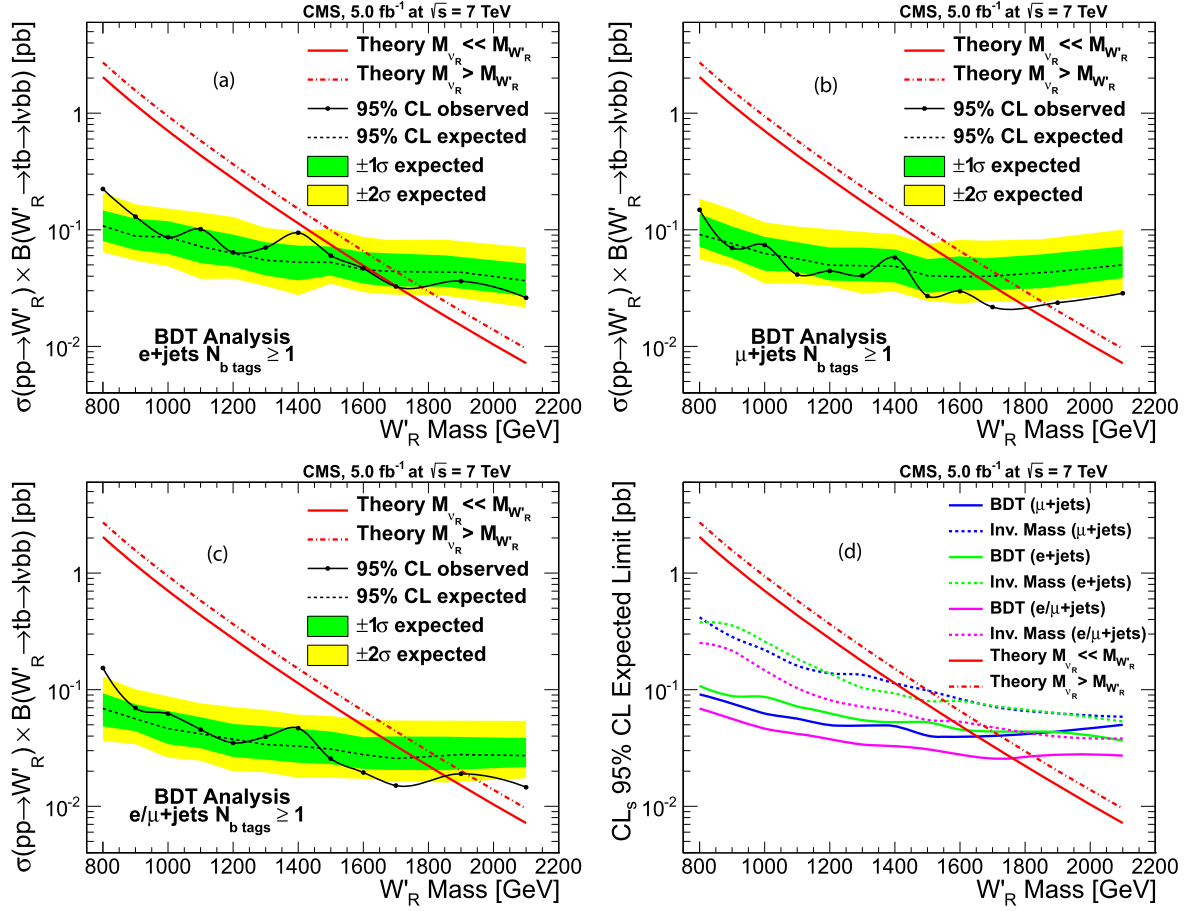
Fig. 4. The expected and measured 95% CL upper limits on the production cross section \sigma(pp \rightarrow W')B(W' \rightarrow tb \rightarrow \ell v b b) of right handed W' bosons obtained using the BDT discriminant for \geq 1 b-tagged electron + jets events (a), muon + jets events (b), and combined (c). Also shown (d) is a comparison of the expected 95% CL upper cross section limits obtained using invariant mass distribution and BDT output for right handed W' bosons for \geq 1 b-tagged muon + jet events, electron + jet events, and combined. The \pm 1\sigma and \pm 2\sigma excursions from expected limits are also shown. The solid and dot-dashed red lines represent the theoretical cross section predictions for the two scenarios M_{\nu_R} > M_{W'} , where W' can decay only to quarks and M_{\nu_R} \ll M_{W'} , where all decays of W' are allowed [16–18]. (For interpretation of the references to color in this figure legend, the reader is referred to the web version of this Letter.)
