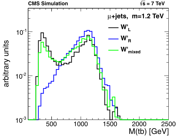
Fig. 1. Simulated invariant mass distributions for production of W'_L , W'_R , and W'_{LR} with a mass 1.2 TeV. For the cases of W'_L and W'_{LR} , the invariant mass distributions also include the contribution from s-channel single top quark production and show a minimum corresponding to the destructive interference between the amplitudes for production of left-handed fermions via the W and W'_L bosons. These distributions are after applying the selection criteria described in Section 4.
