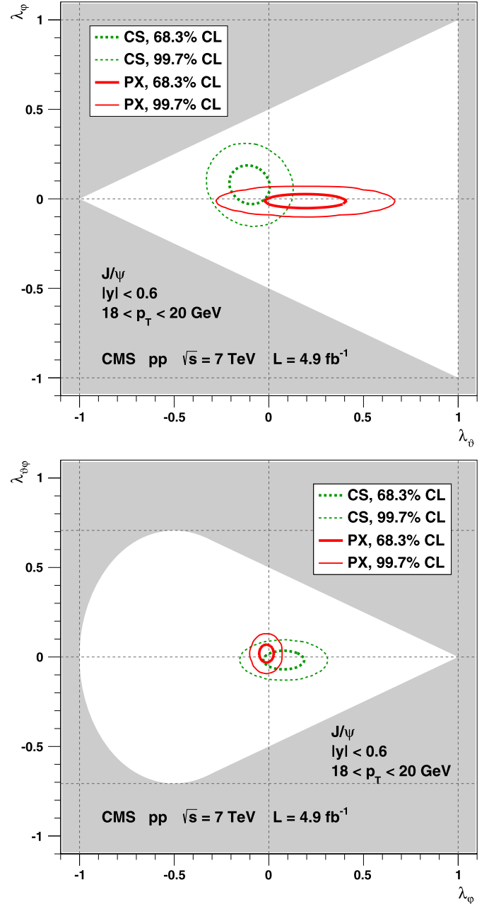
Fig. 5. Two-dimensional marginals of the PPD in the \lambda_\phi vs. \lambda_\theta (top) and \lambda_{\theta\phi} vs. \lambda_\phi (bottom) planes, for J/\psi with |y| < 0.6 and 18 < p_T < 20 GeV. The 68.3% and 99.7% CL total uncertainties are shown for the CS and PX frames. The shaded areas represent physically forbidden regions of parameter space [12].
