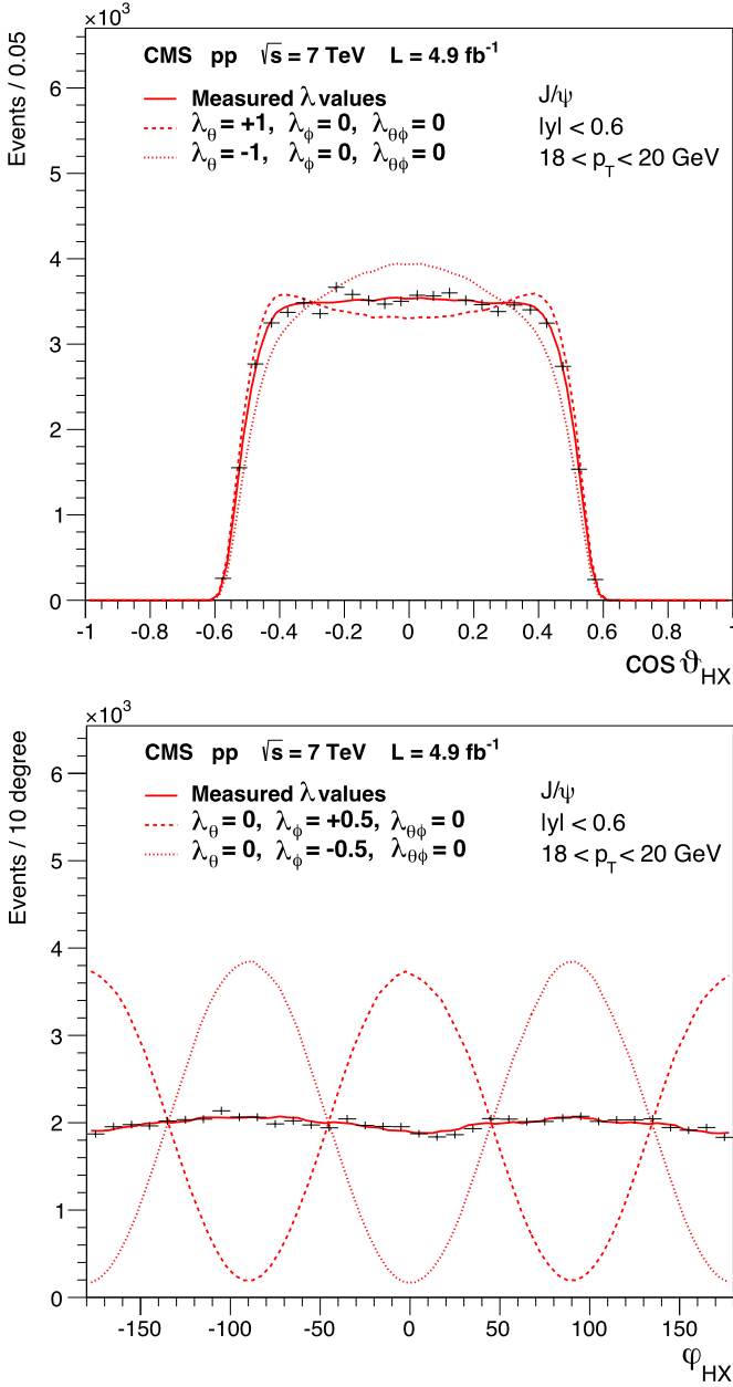
Fig. 4. Frequency distributions of \cos \theta (top) and \varphi (bottom) angular variables, in the HX frame for the J/\psi in an intermediate p_T bin and |y| < 0.6 . The curves represent the expected distributions for two extreme polarization scenarios (dashed and dotted lines defined in the legends) and for the measured \lambda (solid lines).
