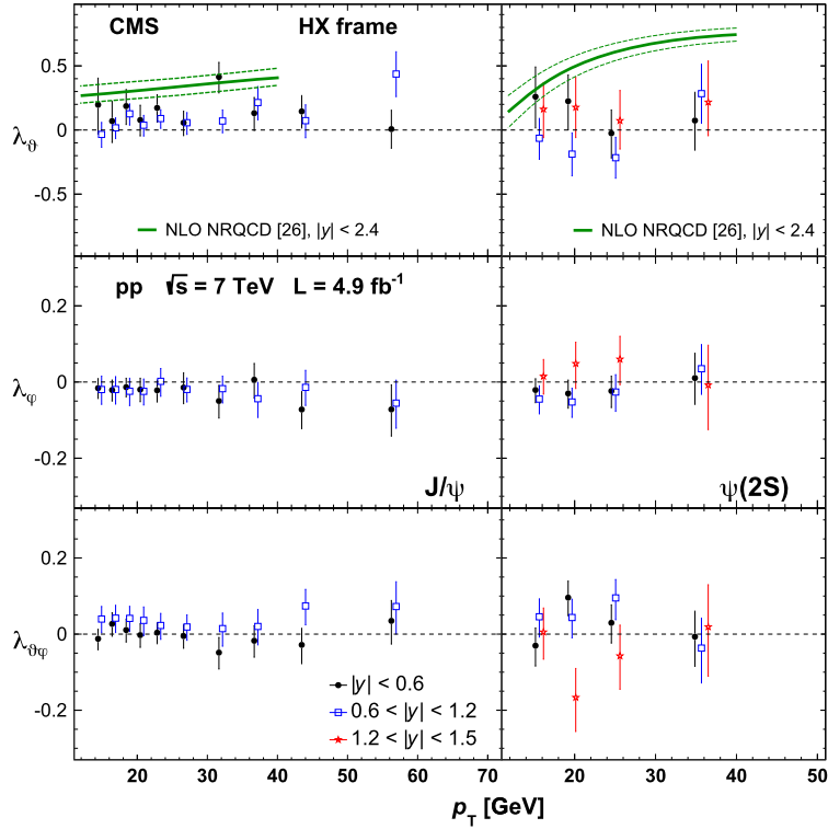
Fig. 6. Polarization parameters \lambda_\theta , \lambda_\phi , and \lambda_{\theta\phi} measured in the HX frame for prompt J/\psi (left) and \psi(2S) (right) mesons, as a function of p_T and for several |y| bins. The error bars represent total uncertainties (at 68.3% CL). The curves in the top two panels represent calculations of \lambda_\theta from NLO NRQCD [26], the dashed lines illustrating their uncertainties.
