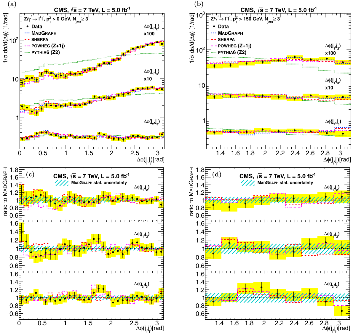
Fig. 6. Normalized \Delta\phi(j_i, j_j) distributions for the inclusive N_{\text{jets}} \geq 3 jet multiplicity bin: (a) all p_T^Z and (b) p_T^Z > 150 \text{ GeV} . Plots in (c) and (d) show the ratios of the data and other MC predictions, relative to MADGRAPH, as described in Fig. 4.
