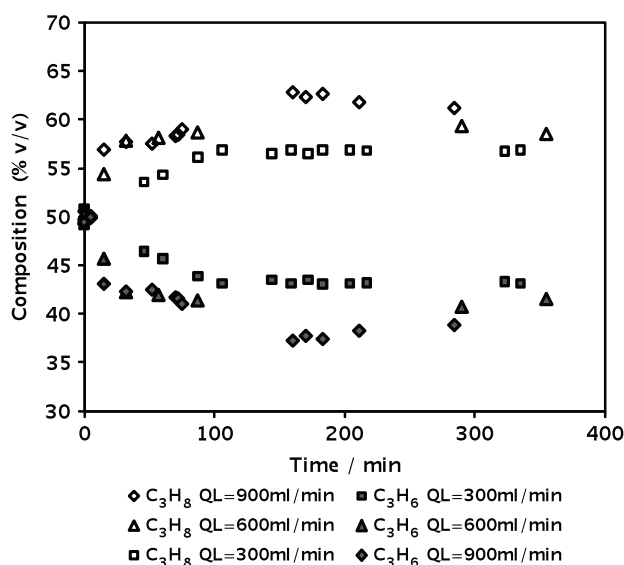
Fig. 1. Evolution of the outlet gas stream compositions in the membrane module versus time for constant inlet gas flow rate (50–50 % v/v C_3H_6 – C_3H_8 ) at 298 K and different liquid volumetric flow rate Q_L .
