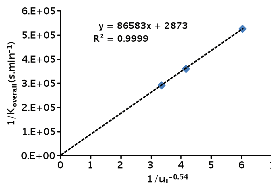
Fig. 2. Wilson plot – effect of velocity of absorbing liquid on overall mass transfer coefficient.
