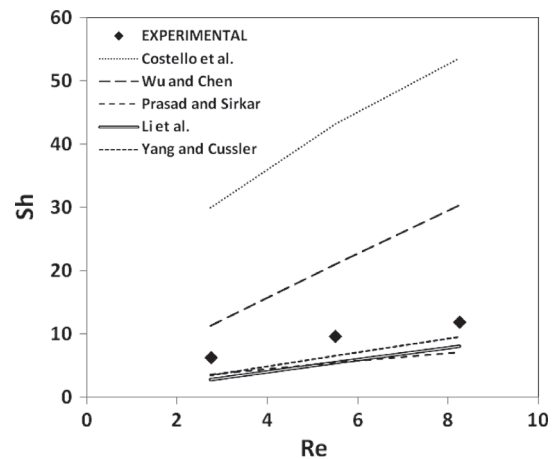
Fig. 3. Comparison between experimental results and reported correlations.
