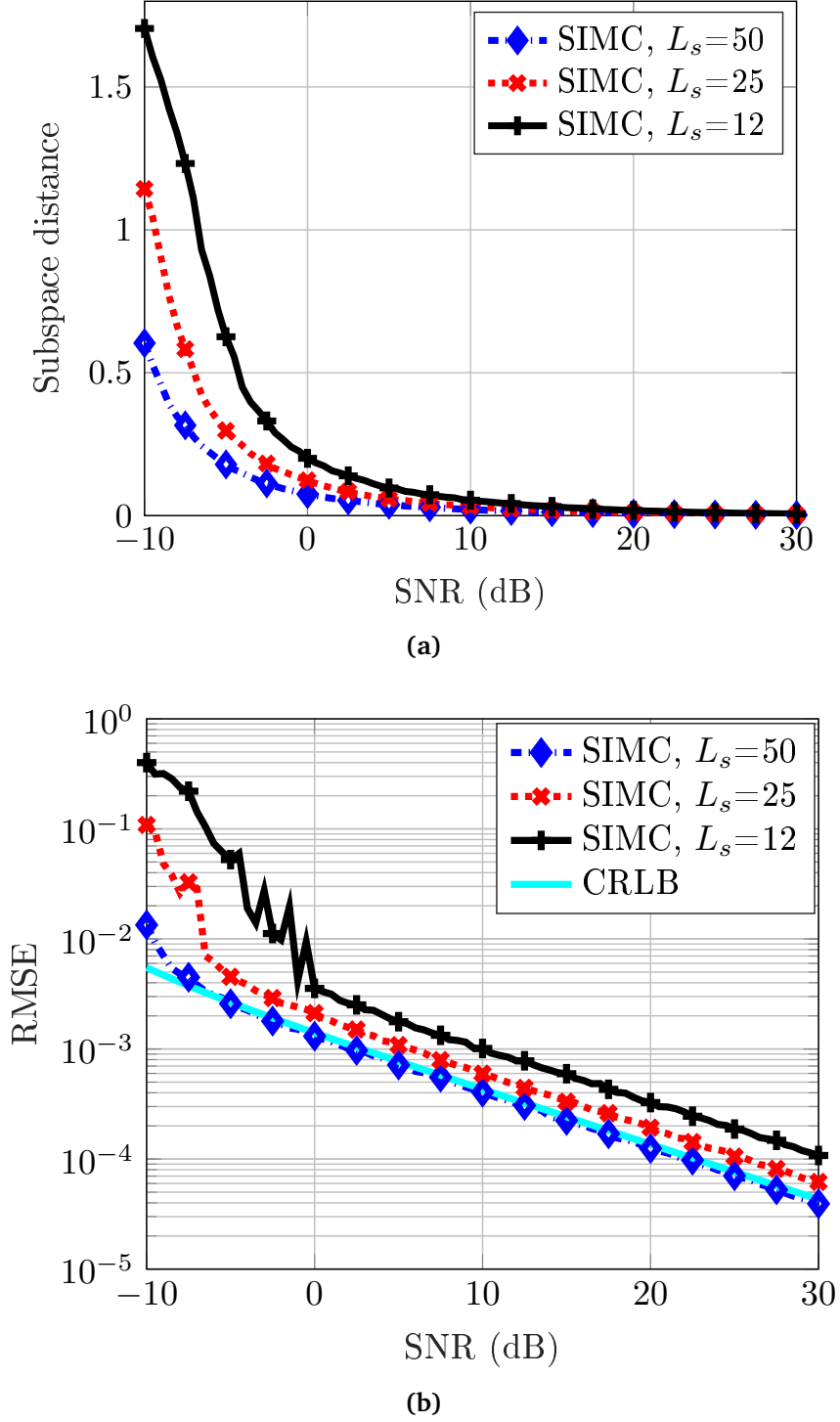
Figure 5.6: Subspace distance (a) and RMSE (b) vs. SNR when M = 50 , N = 80 , K = 3 and \Delta_\theta = 10^\circ for L_s = (50, 25, 12) .
