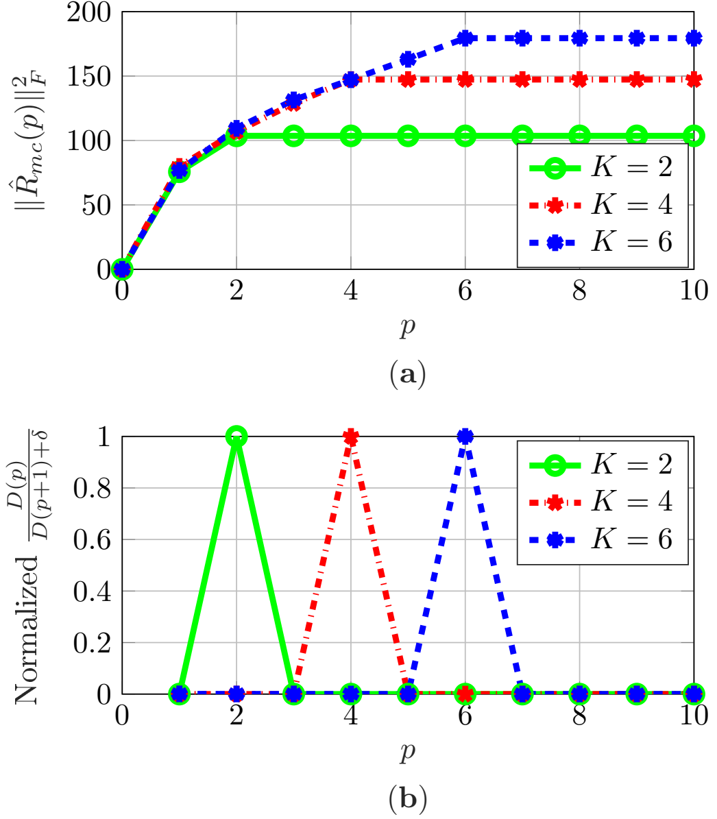
Figure 4.1: (a) \|\hat{\mathbf{R}}_{mc}(p)\|_F^2 vs. p , and (b) Normalized \frac{D(p)}{D(p+1)+\delta} vs. p for M = 100 , N = 150 , \epsilon_d = 0.5 , \text{SNR} = -10 dB and sources are separated by 10^\circ .
