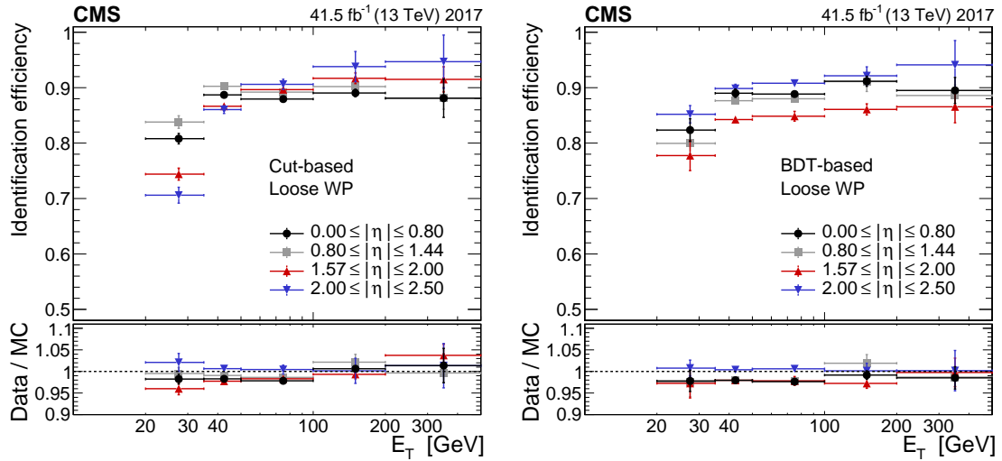
Figure 27. Photon identification efficiency in data (upper panels) and data-to-simulation efficiency ratios (lower panels) for the loose cut-based (left) and loosest BDT-based (right) identification working points, as functions of the photon E_T . The vertical bars on the markers represent combined statistical and systematic uncertainties.
