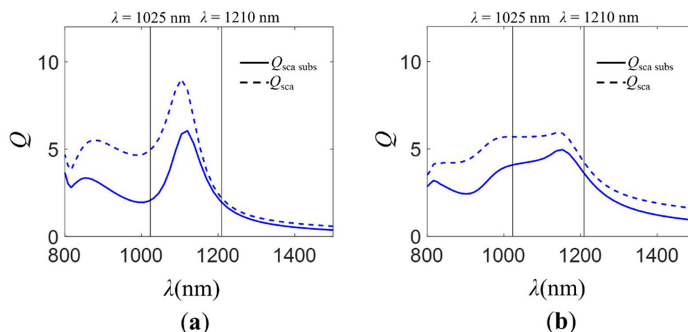
Figure 5. Total normalized scattering cross-section, Q_{\text{sca}} (dashed line), and normalized scattering cross-section for radiation scattered into the substrate, Q_{\text{sca subs}} (solid line), for different configurations of HRID particles on a graded-index multilayer substrate. (a) Isolated silicon NP of radius R = 150 nm. (b) Dimer of silicon NPs of radius R = 150 nm and gap distance d = 10 nm. The substrate consists of two dielectric layers of thicknesses ( t ) and refractive indices ( n ) t_1 = 185 nm, t_2 = 104 nm and n_1 = 1.396 and n_2 = 2.474 , respectively, on a silicon layer ( n_s = 3.5 ). The structures were illuminated by an unpolarized plane wave propagating normally to the surface of the substrate. Vertical black lines correspond to the wavelengths where the zero-backward ( \lambda = 1210 nm) and near zero-forward/“near zero-backward” ( \lambda = 1025 nm) conditions are attained.
