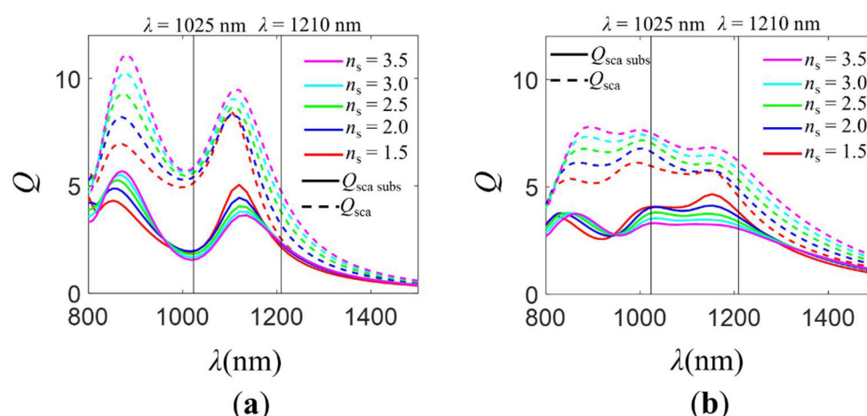
Figure 3. Total normalized scattering cross-section, Q_{\text{sca}} (dashed line), and normalized scattering cross-section for radiation scattered into the substrate, Q_{\text{sca subs}} (solid line), for different configurations of silicon NPs. (a) Isolated silicon NP of radius R = 150 nm. (b) Dimer of silicon NPs of radius R = 150 nm and gap distance d = 10 nm. The NPs were located on the surface of a monolayer substrate of known optical properties. The refractive index of the substrate was varied, n_s \in [1.5\text{--}3.5] . The structures were illuminated by an unpolarized plane wave propagating normally to the surface of the substrate. Vertical black lines correspond to the wavelengths where the zero-backward ( \lambda = 1210 nm) and near zero-forward/“near zero-backward” ( \lambda = 1025 nm) conditions were attained.
