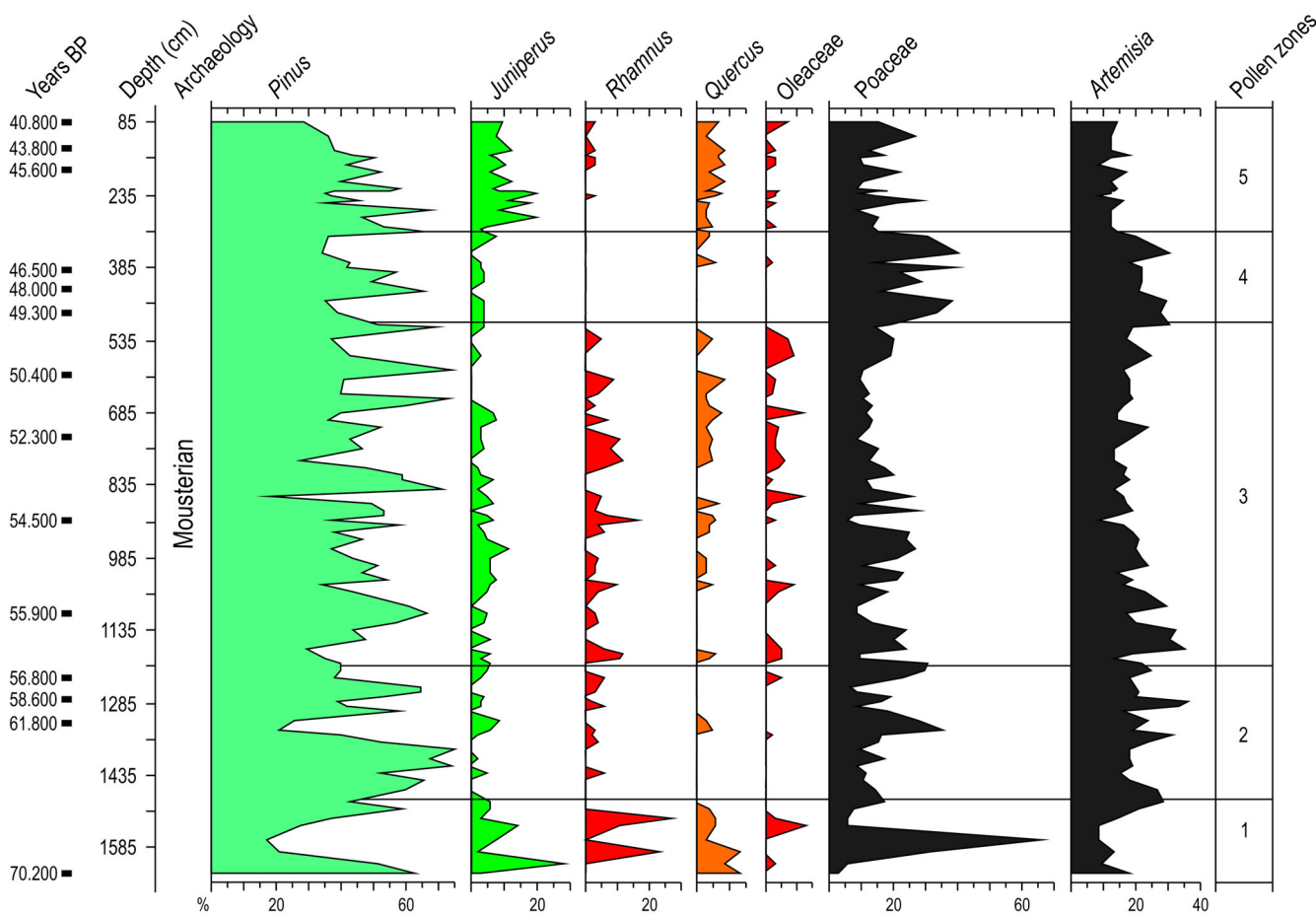
Figure 10. Main pollen curves and chronology of the Upper Pleistocene Romaní cave sequence (Burjachs and Julià, 1994). [Color figure can be viewed at wileyonlinelibrary.com ]
