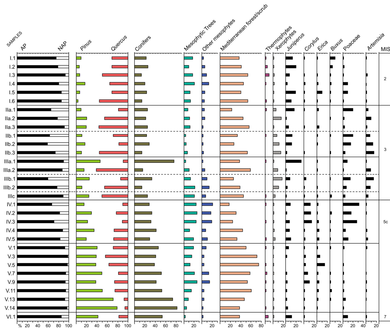
Figure 7. Synthetic pollen diagram of selected taxa from Teixoneres Cave. Redrawn from Ochando et al. (2020a). [Color figure can be viewed at wileyonlinelibrary.com ]
