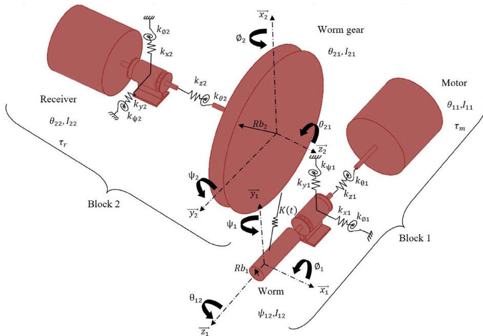
Figure 1. The dynamic model of the worm drive.
