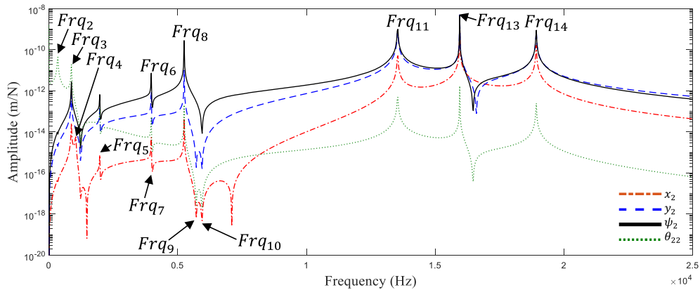
Figure 4. Frequency response function (FRF) of x_2 , y_2 , \psi_2 , and \theta_{22} .
