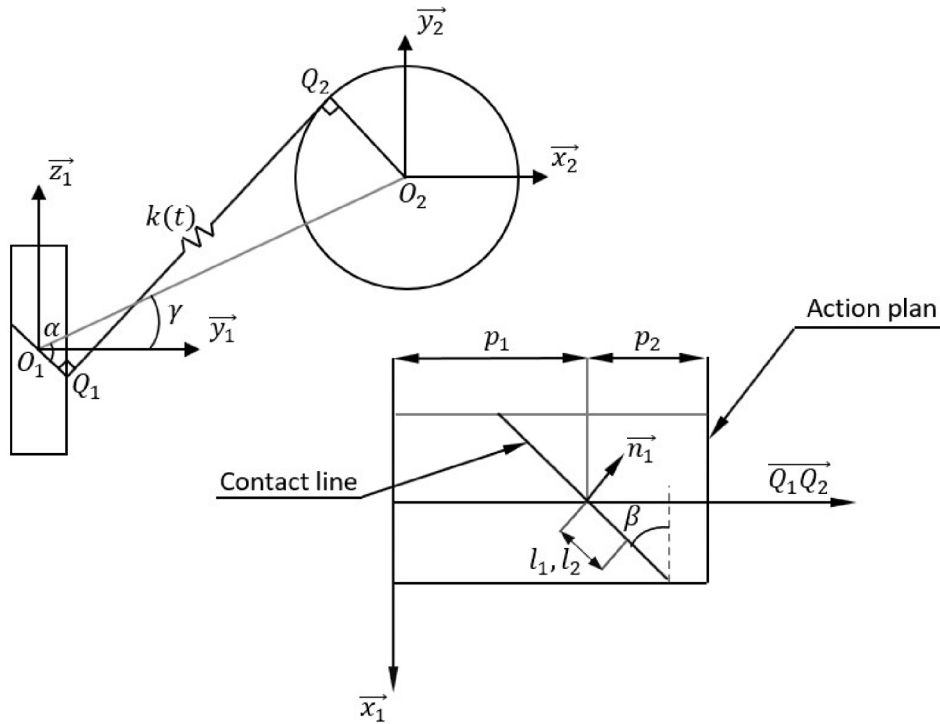
Figure 2. Modelling of the teeth contact of the gears.
