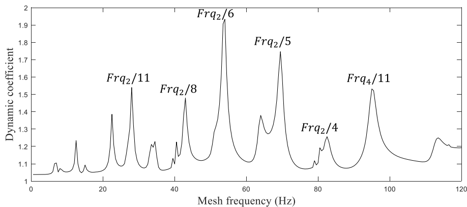
Figure 11. Evolution of the dynamic coefficient.
