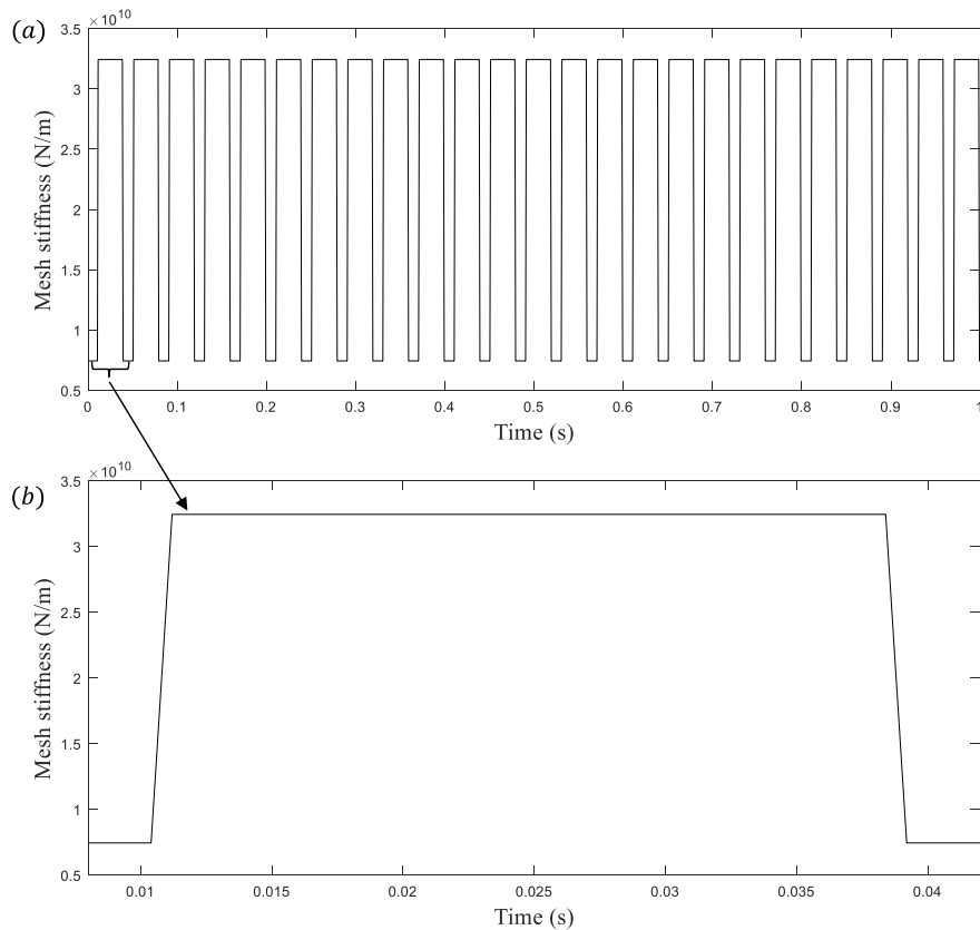
Figure 8. (a) Multiple and (b) single gear mesh stiffness against a time frame.
