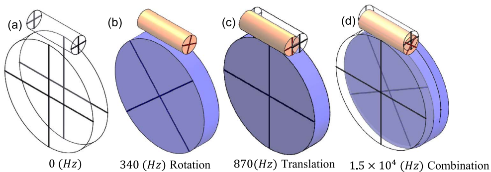
Figure 5. Examples of different mode shapes.
