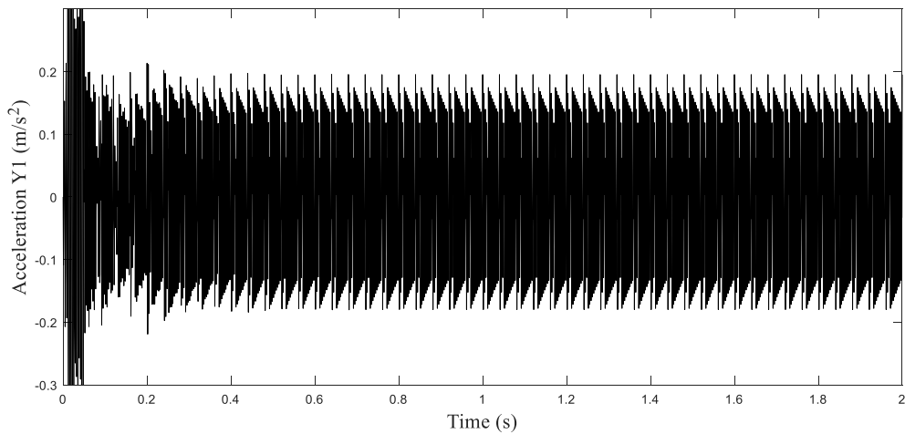
Figure 9. The time-dependent acceleration of the worm.
