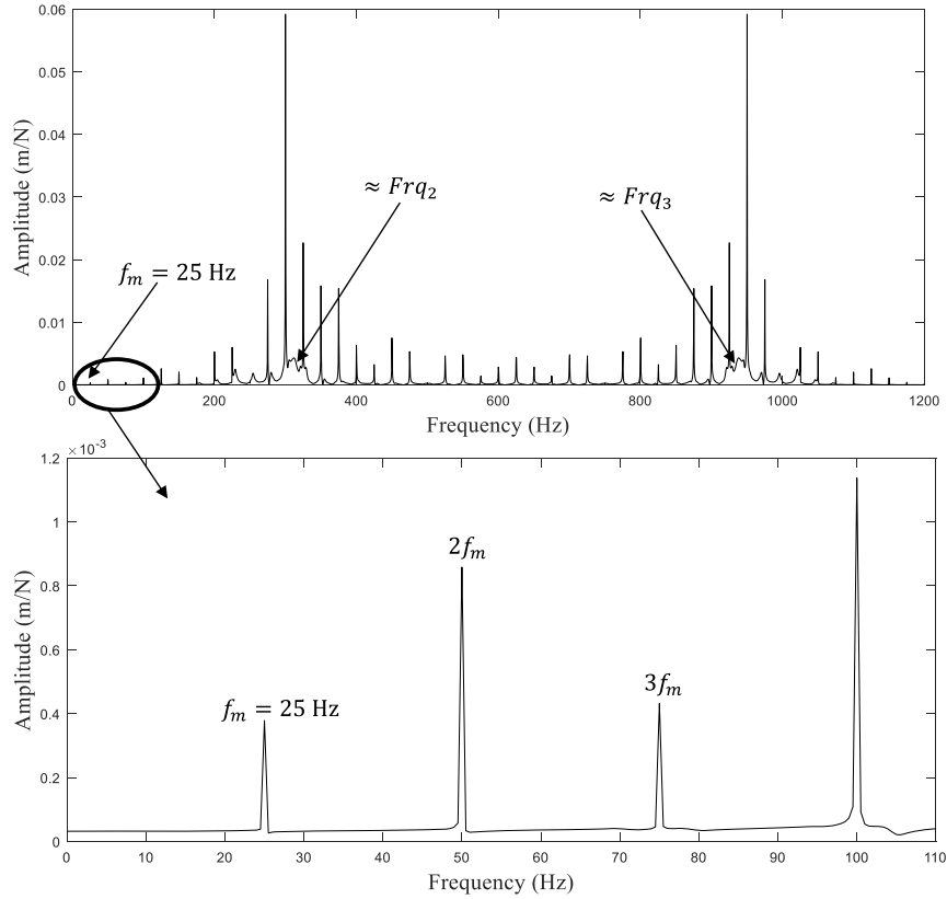
Figure 10. Spectrum the acceleration of the worm.
