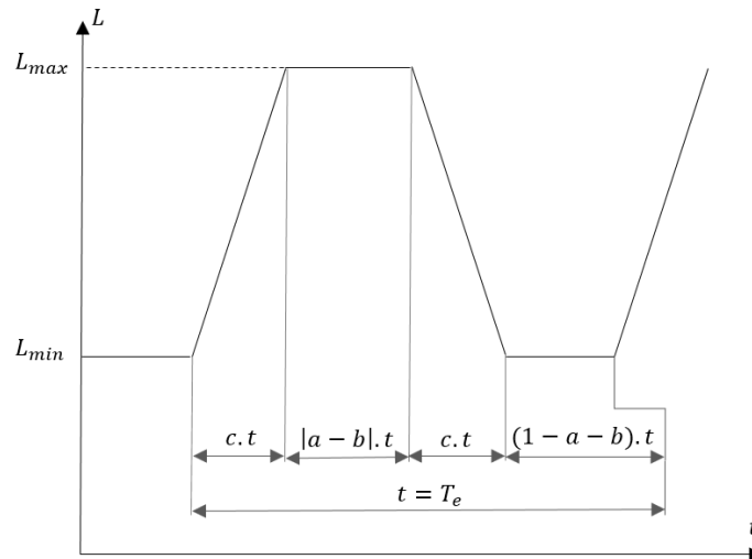
Figure 3. Evolution of the length of the line of action.
