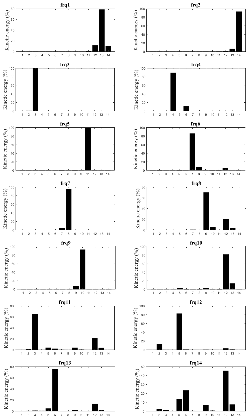
Figure 7. Kinetic energy distribution.
