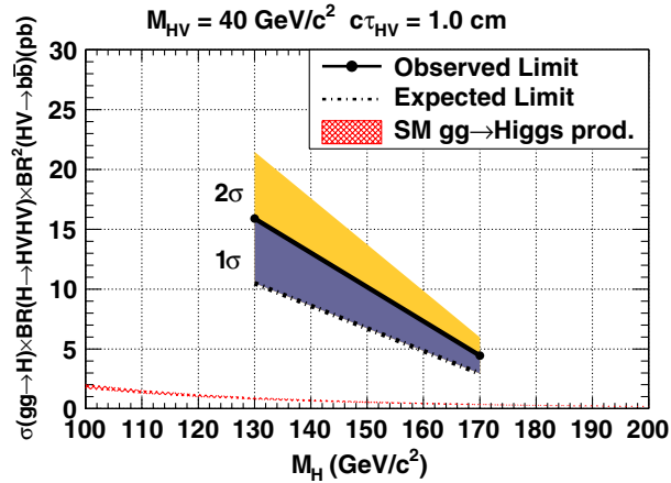
FIG. 10 (color online). Observed and expected limits at 95% C.L. with +1 and +2 \sigma bands for signal MC with HV masses 40 GeV/c 2 . The hashed line is the Higgs boson production cross section in the SM.
