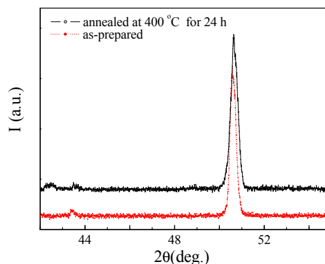
Figure 23. XRD patterns of as-prepared and annealed at 400 °C for 24 h Cu 90 Co 10 microwires.
