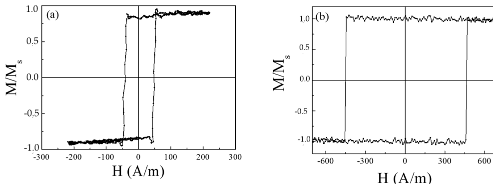
Figure 3. Hysteresis loops of as-prepared Fe 70.8 Cu 1 Nb 3.1 Si 16 B 9.1 microwires with \rho = 0.62 (a) and as-prepared Fe 38.5 Co 38.5 B 18 Mo 4 Cu 1 with \rho = 0.60 (b). Reproduced from reference [10], Figure 5.
