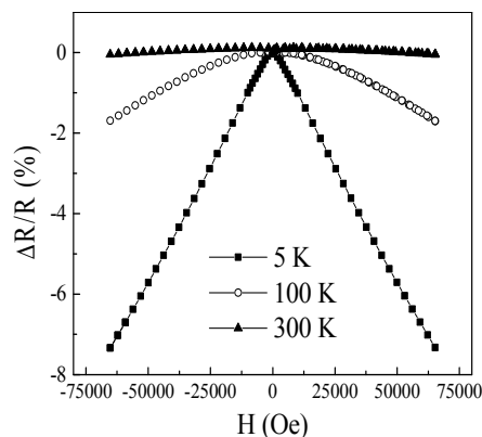
Figure 29. Magnetoresistance of the as-cast \text{Cu}_{63}\text{Fe}_{37} microwire with \rho = 0.31 measured at 5 K, 100 K and 300 K at magnetic field from -70 to 70 kOe. Reproduced from reference [92], Figure 5.
