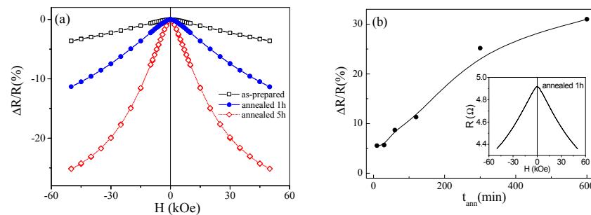
Figure 20. Effect of annealing ( T_{\text{ann}} = 400 °C) on GMR effect of \text{Cu}_{90}\text{Co}_{10} microwires (a) and dependence of GMR effect on annealing time (b). Real resistance variation with magnetic field in the sample annealed at 400 °C for 1 h measured at 5 K is shown in the inset of Figure 2b.
