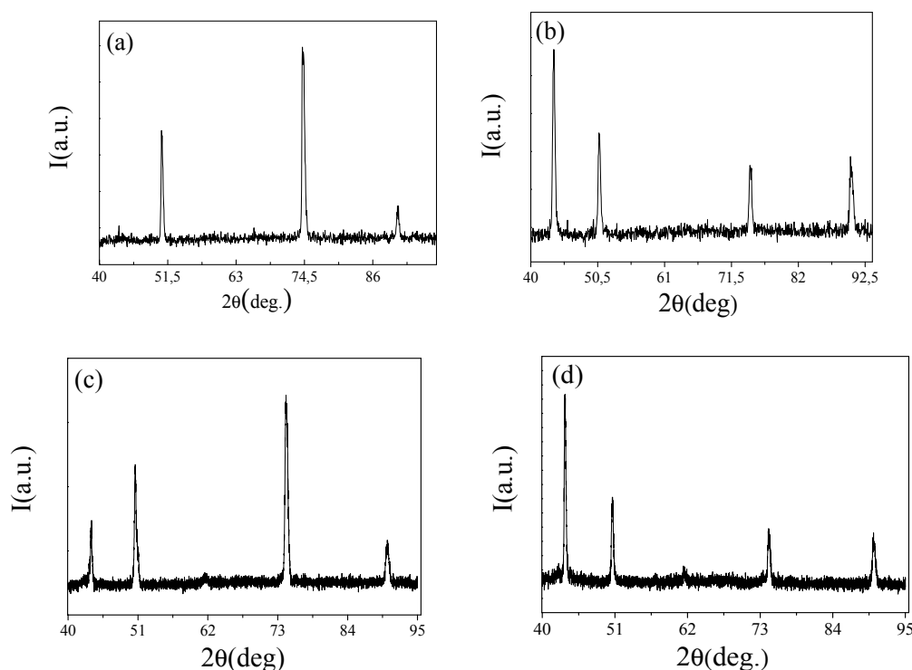
Figure 22. XRD of as-prepared (a,b) and annealed at T_{\text{ann}} = 400\text{ }^{\circ}\text{C} for 24 h (c,d) \text{Cu}_{95}\text{Co}_5 and \text{Cu}_{80}\text{Co}_{20} microwires respectively. Reproduced from reference [85], Figure 2.
