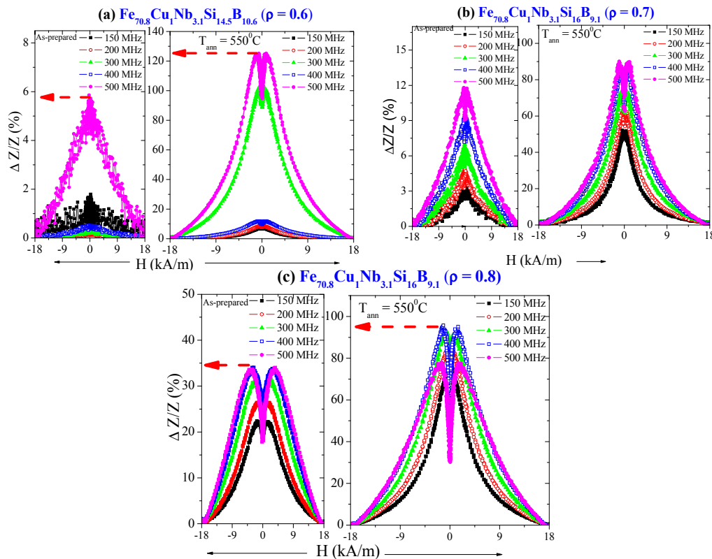
Figure 9. \Delta Z/Z (H) of as-prepared and annealed \text{Fe}_{70.8}\text{Cu}_1\text{Nb}_{3.1}\text{Si}_{14.5}\text{B}_{10.6} at T_{\text{ann}} = 550^\circ\text{C} for \rho -ratio = 0.6 (a); \Delta Z/Z (H) of \text{Fe}_{70.8}\text{Cu}_1\text{Nb}_{3.1}\text{Si}_{16}\text{B}_{9.1} for \rho -ratio = 0.7 (b); and \rho -ratio = 0.8 (c). Driving frequencies are provided in each figure. Reproduced from reference [47], Figure 6.
