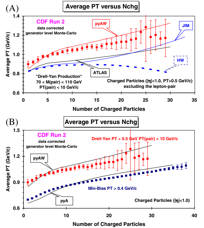
FIG. 15 (color online). (a) CDF data at 1.96 TeV on the average p_T of charged particles versus the multiplicity for charged particles for Drell-Yan events in which p_T(\text{lepton-pair}) < 10 GeV/c. The data are compared with PYTHIA Tune AW (pyAW), the PYTHIA ATLAS tune, HERWIG without MPI (HW), and HERWIG with JIMMY MPI (JIM). (b) Comparison of the average p_T of charged particles versus the charged multiplicity for min-bias events from Ref. [20] with the Drell-Yan events with p_T(\text{lepton-pair}) < 10 GeV/c from this analysis. The min-bias data require p_T > 0.4 GeV/c and are compared with PYTHIA Tune A (pyA), while the Drell-Yan data require p_T > 0.5 GeV/c and are compared with PYTHIA Tune AW (pyAW).
