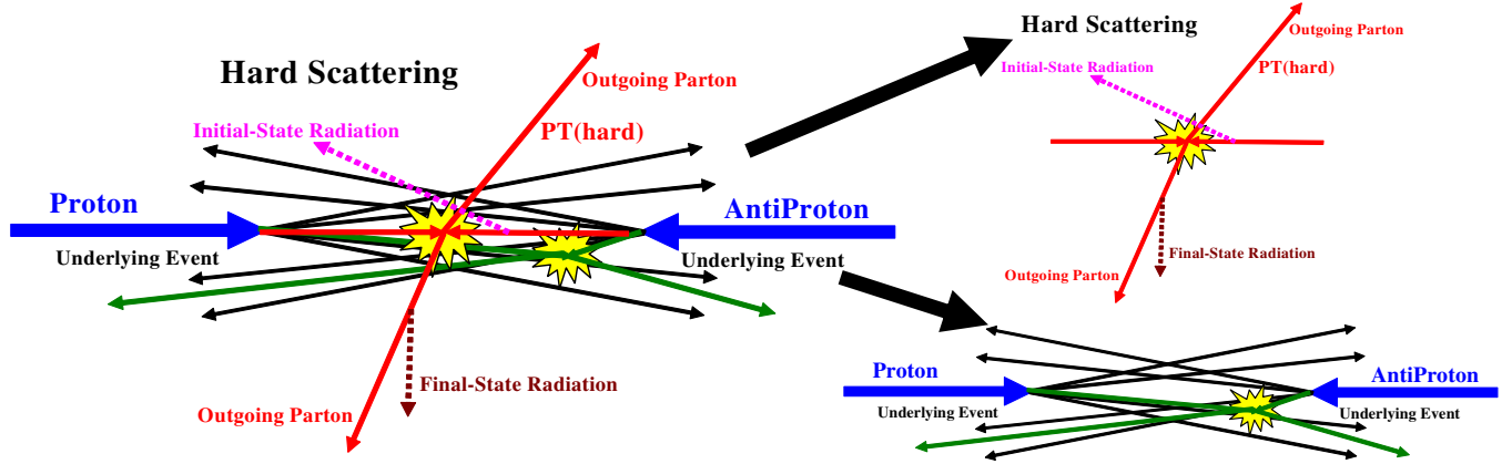
FIG. 1 (color online). Illustration of the way QCD Monte Carlo models simulate a proton-antiproton collision in which a hard two-to-two parton scattering with transverse momentum, p_T(\text{hard}) , has occurred. The hard-scattering component of the event consists of particles that result from the hadronization of the two outgoing partons (i.e. the initial two jets) plus the particles that arise from initial and final-state radiation (i.e. multijets). The underlying event consists of particles that arise from the beam-beam remnants and from multiple-parton interactions.
