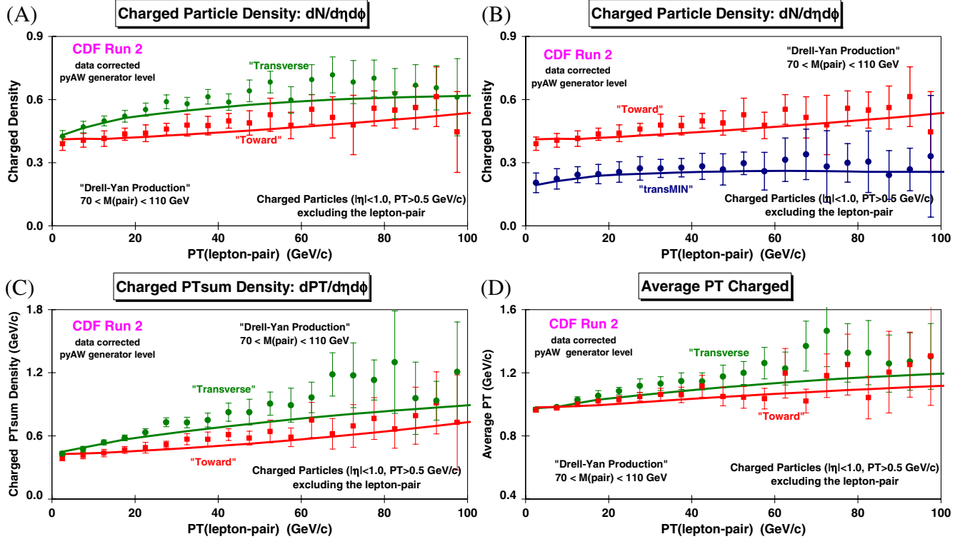
FIG. 11 (color online). (a) Compares the CDF data at 1.96 TeV on the charged-particle density in the toward and transverse regions for Drell-Yan events. Also shows the predictions of PYTHIA Tune AW. (b) Compares the CDF data on the charged-particle density in the toward and transMIN regions for Drell-Yan events and also shows the predictions of PYTHIA Tune AW. (c) The same as (a) for the scalar PT_{\text{sum}} density. (d) The same as (a) for the average charged-particle p_T of charged particles.
