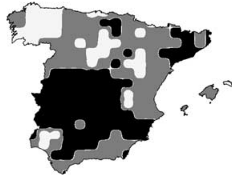
Fig. 13. Regions of Spain (interpolated from the 203 mesh) where the difference between the observation and forecast differ less than 20 percentiles in two (black), one (dark grey) and zero (light grey) cases out of the two NDJ seasons for the ECMO18AN in the period 1986–1987.
