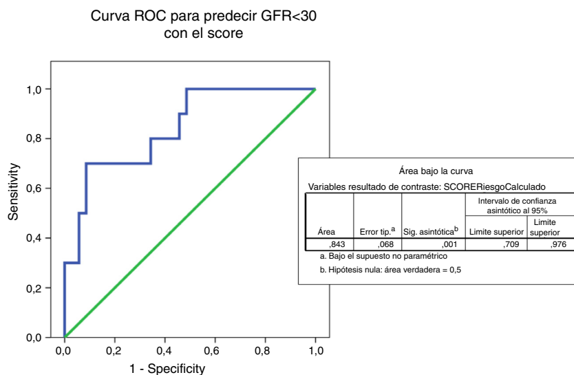
Figure 5 – ROC curve to analyze the ability of the test to predict an eGFR of less than 30 ml/min based on the IgANPC score. AUC = 0.843.
