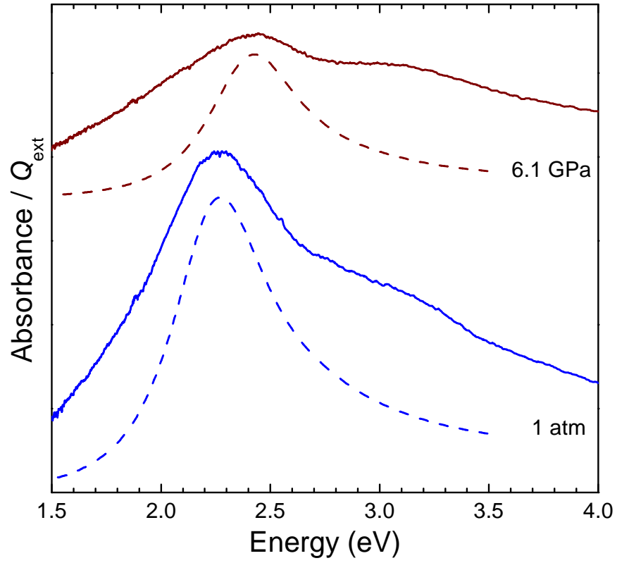
Figure 3: Experimental (continuous line) and calculated by Mie theory (dashed line) absorbance spectra of irradiated \text{CaF}_2 at ambient temperature and P = 1 atm and 6.1 GPa.
