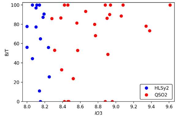
Figure 5. Relative contribution of the spheroidal component to the total galaxy light (B/T) versus IO3 . Only galaxies that could be fitted with GALFIT are plotted. B/T increases with AGN power. For IO3 \gtrsim 8.6 , most galaxies are bulge-dominated.
