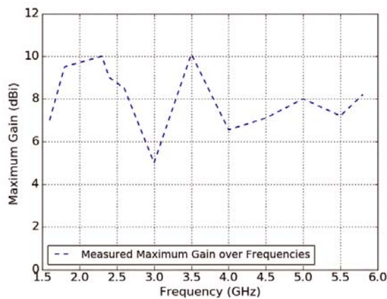
Figure 11. The maximum gain measurements over frequency.
