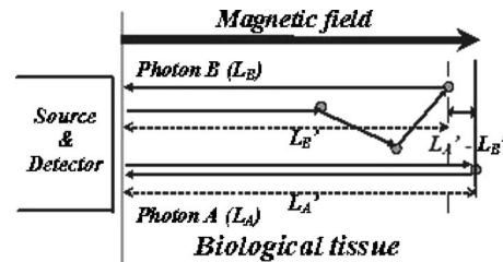
Fig. 1 Two photons A and B simultaneously arriving at the detector travel the same optical path lengths ( L_A = L_B ) but traverse different path lengths ( L'_A, L'_B ) in the direction of the external magnetic field, thus encountering different polarization rotations.
