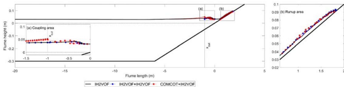
Figure 8. Comparison among the IH2VOF model and the numerical flume. Subplots of the coupling and the run-up areas are depicted.
