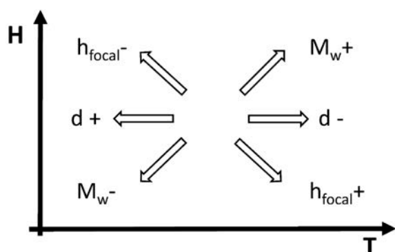
Figure 9. General scheme of the tsunami wave height ( H ) and period ( T ) behavior in relation to the water depth ( d ) in the generation area and earthquake focal depth ( h_{\text{focal}} ) and magnitude ( M_w ).
