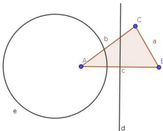
Figure 15 A generalization of the bisector
