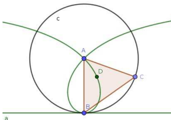
Figure 7 A strophoid
