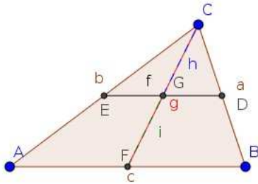
Figure 20 A property of the midline
