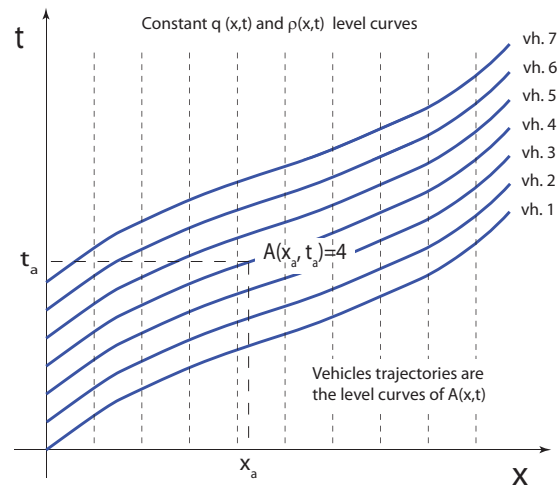
Figure 4.25: Illustration of the vehicle trajectories (level curves of the A(x, t) function).
