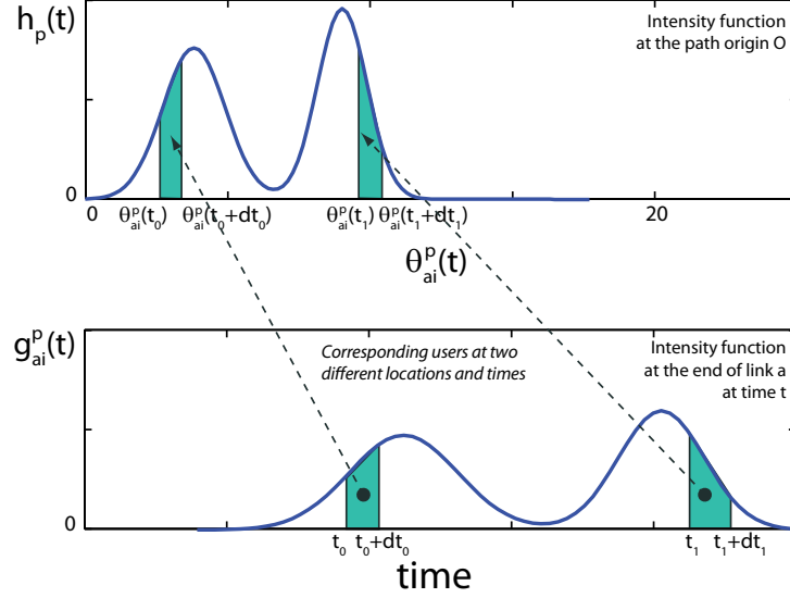
Figure 7.5: Illustration of how the traffic wave satisfies the flow propagation principle and the function \theta_a^p(t) .
