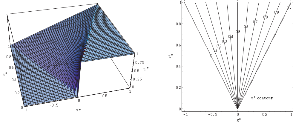
Figure 4.15: u^*(x^*, t^*) contours.
