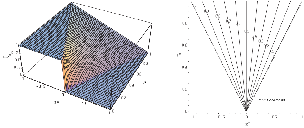
Figure 4.14: \rho^*(x^*, t^*) contours.
