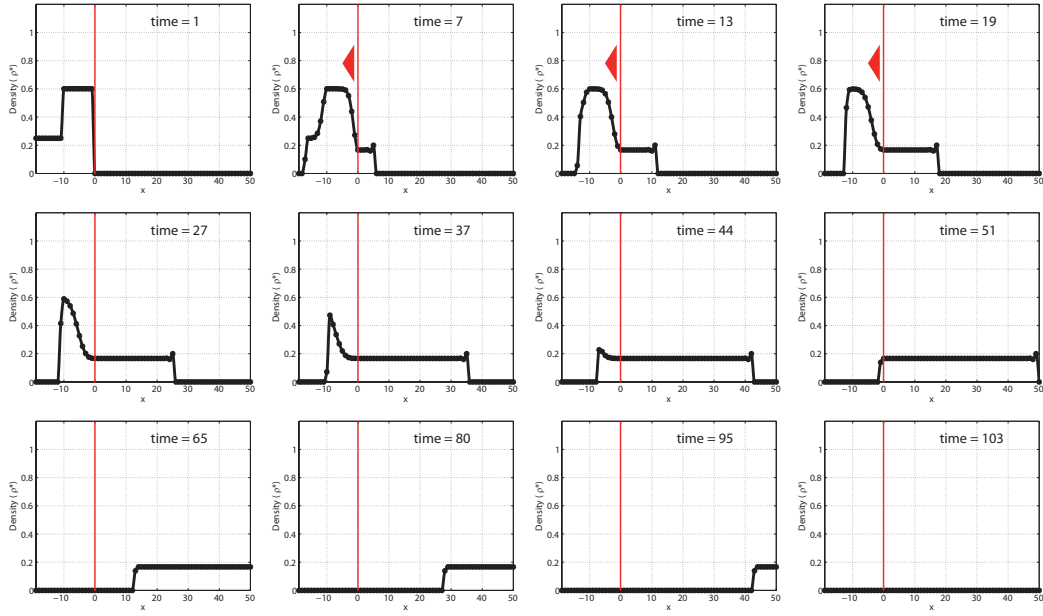
Figure 4.13: Time evolution of flow density (CTM). Case (a): \rho_1^* = 0.60 and \rho_2^* = 0.25 , with w/v = 0.20 .
