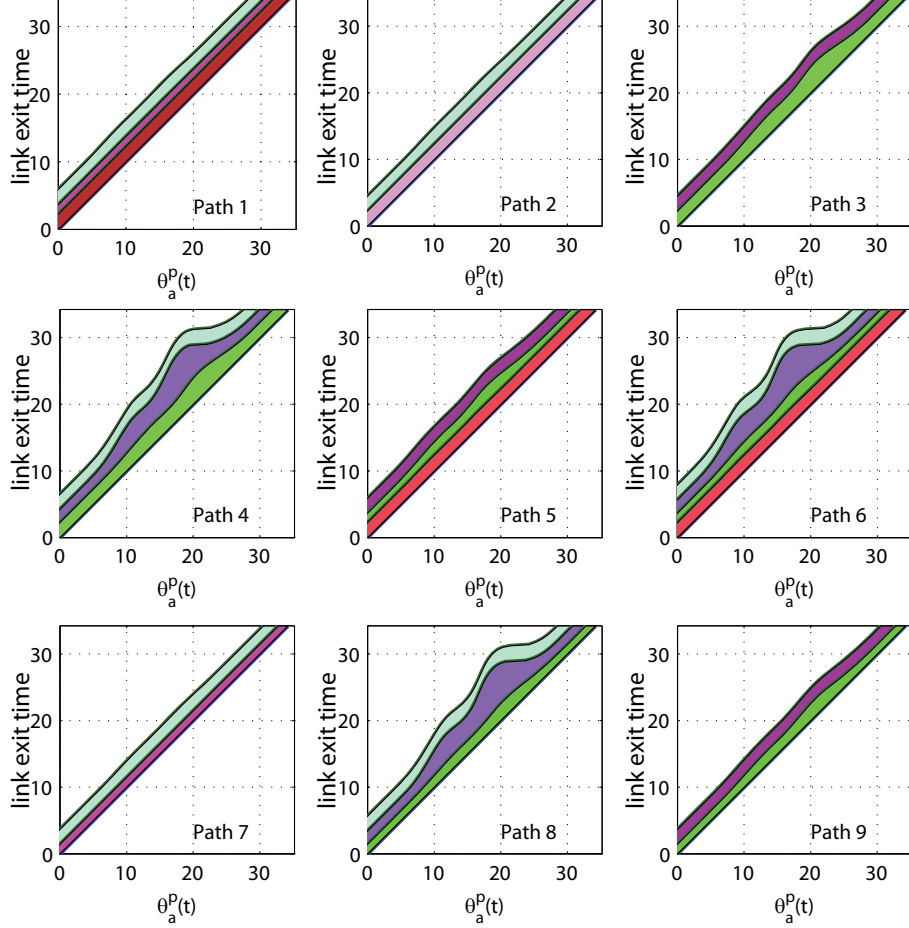
Figure 7.12: Illustrative example. Link exit time functions obtained by adding the departure time function f(t) = t and the corresponding link travel time functions for all paths with the corresponding link.
