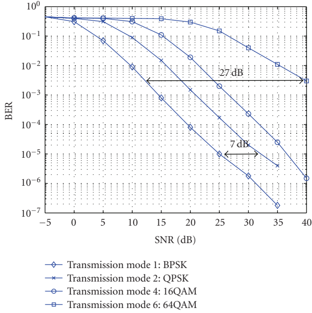
FIGURE 12: BER comparison for different IEEE 802.16 transmission modes using 2 \times 2 MIMO.
