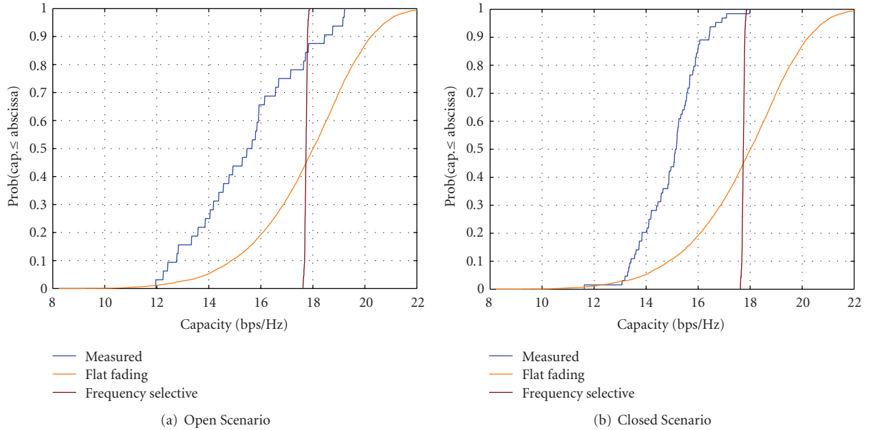
FIGURE 9: The MIMO channel capacity with SNR = 30 dB measured and modeled in NLOS areas.
