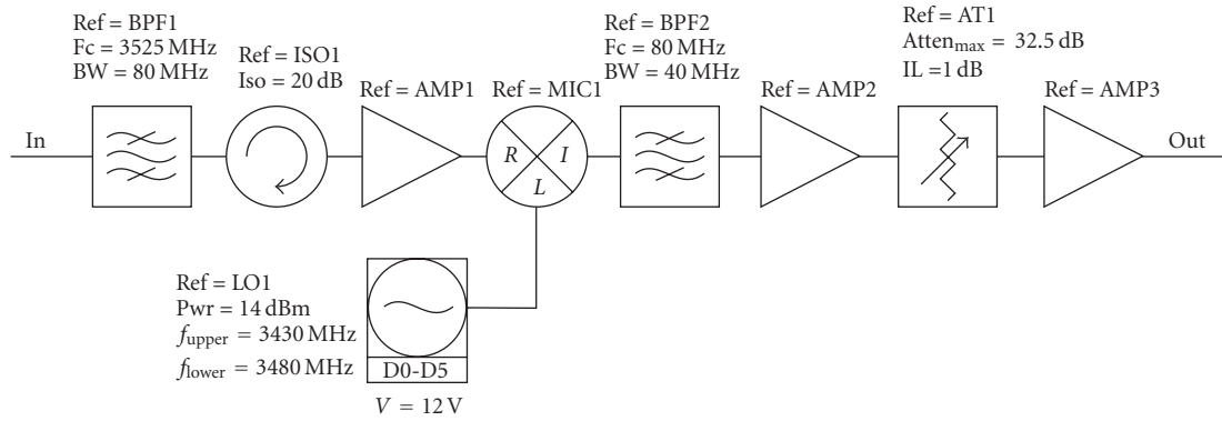
FIGURE 3: Radio Frequency Chain RX Modules Diagram.
