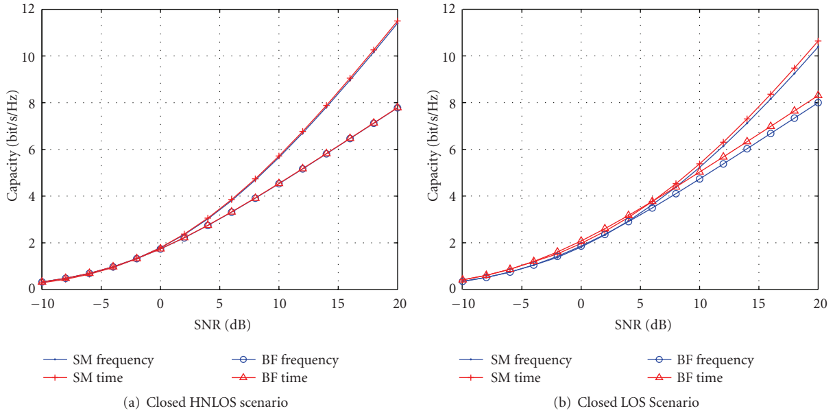
FIGURE 11: Average Capacity with frequency averaging versus time averaging.
