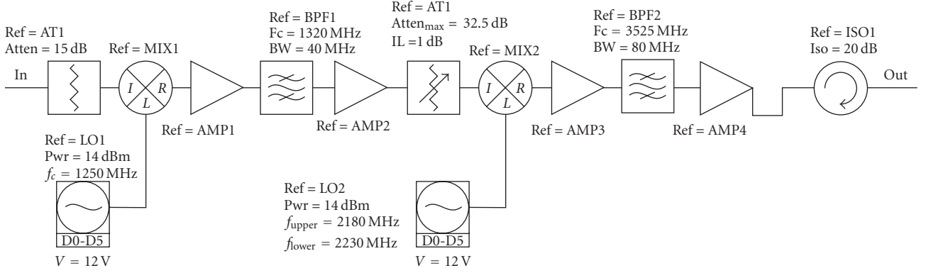
FIGURE 2: Radio Frequency TX Chain Modules Diagram.
