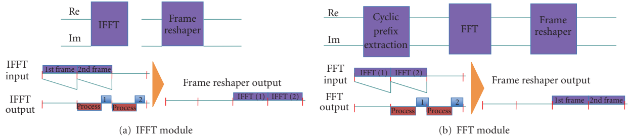
FIGURE 6: IFFT/FFT Reshaping module.
