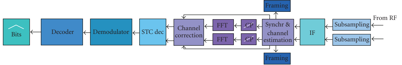
FIGURE 5: Base-Band and IF Receiver Block diagram.
