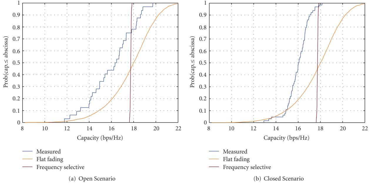
FIGURE 10: The MIMO channel capacity with SNR = 30 dB measured and modeled in HNLOS areas.
