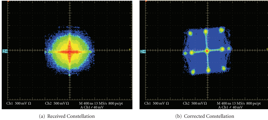
FIGURE 7: Constellations for QPSK at Antenna 1 at SNR = 20 dB.
