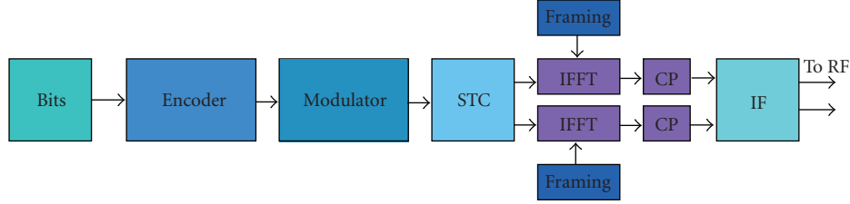
FIGURE 4: Base-Band and IF Transmitter Block diagram.
