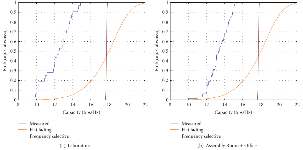
FIGURE 8: CDF of the MIMO channel capacity with SNR = 30 dB measured and modeled in LOS areas.
