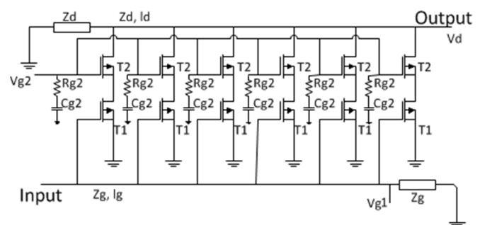
Fig. 1. Electrical schematic for the distributed amplifier.
