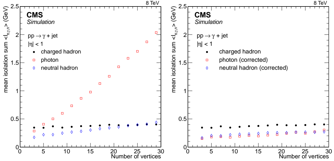
Figure 16. Mean value of the isolation variables for photons with p_T > 50 GeV in \gamma +jet events, as a function of the number of reconstructed primary vertices, for events (left) before and (right) after being corrected for pileup using the \rho variable.
