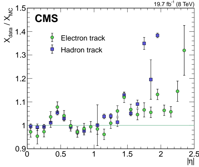
Figure 9. Tracker material thickness (in terms of radiation lengths) inferred in the data, X_{\text{data}} , relative to that inferred in simulated events, X_{\text{MC}} , as a function of |\eta| , using electrons in Z \rightarrow e^+e^- events (circles), and low-momentum charged hadrons (squares).
