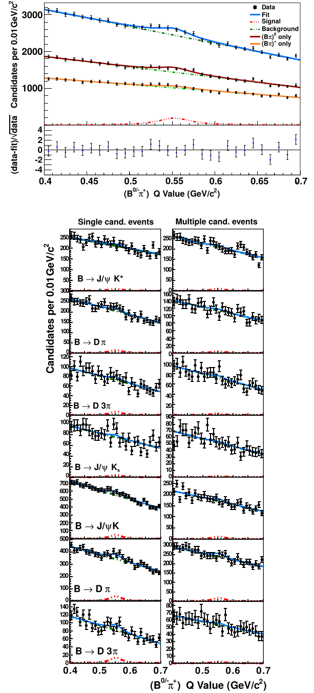
FIG. 7 (color online). Spectra of the Q value of B^{*0,+} candidates in all the considered decay channels with fit results for the broad structure overlaid. The upper panel shows the data summed over decay channels and the deviations of these from the fit function, normalized to the Poisson uncertainty of the data. The lower plot shows the simultaneously fit spectra separately.
