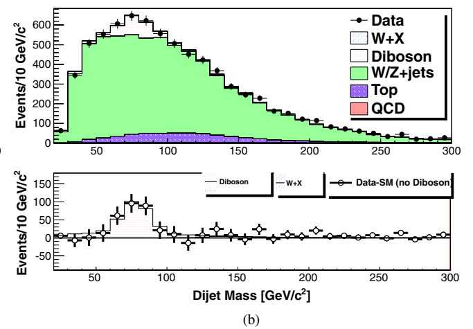
FIG. 12 (color online). Dijet mass distribution with fit results overlaid in the electron (a) and muon data sets (b) incorporating improved jet-energy-scale corrections for simulated quark and gluon jets but no tuning on the multijet-background modeling. The bottom panel shows data with all fit background contributions subtracted except those from diboson production.
