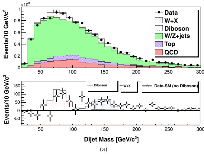
FIG. 11 (color online). Same distribution as in Fig. 10 shown separately for the electron (a) and muon (b) samples.
