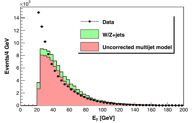
FIG. 3 (color online). Transverse-energy distribution of jets matched to identified electrons in the multijet-enriched control region in data (circles), uncorrected multijets model (dark shaded histogram), and W/Z + \text{jets} simulation (light shaded histogram). The magnitude of W/Z + \text{jets} contributions is normalized to the NLO calculations [23], while the magnitude of the multijet model is obtained from the data. In subsequent analysis, the multijet model is reweighted such that the predicted and observed energy spectra agree.
