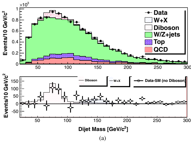
FIG. 12 (color online). Dijet mass distribution with fit results overlaid in the electron (a) and muon data sets (b) incorporating improved jet-energy-scale corrections for simulated quark and gluon jets but no tuning on the multijet-background modeling. The bottom panel shows data with all fit background contributions subtracted except those from diboson production.
