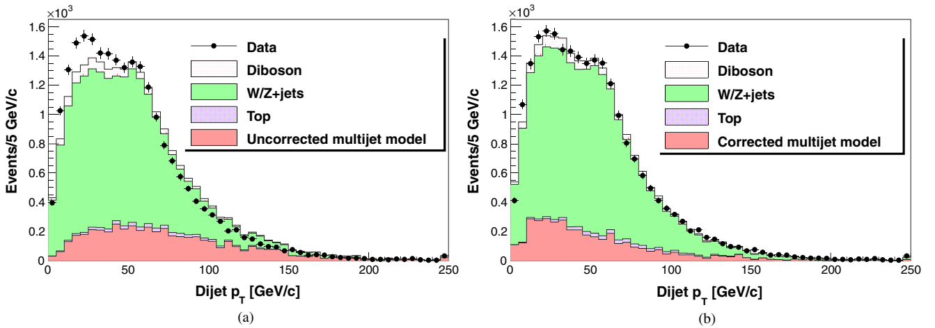
FIG. 5 (color online). Transverse-momentum distribution of the two-jet system in the selected event sample with looser selection criteria as observed in the data and as predicted by the models before (a) and after (b) application of tunings to the nonelectron-based multijet model.
