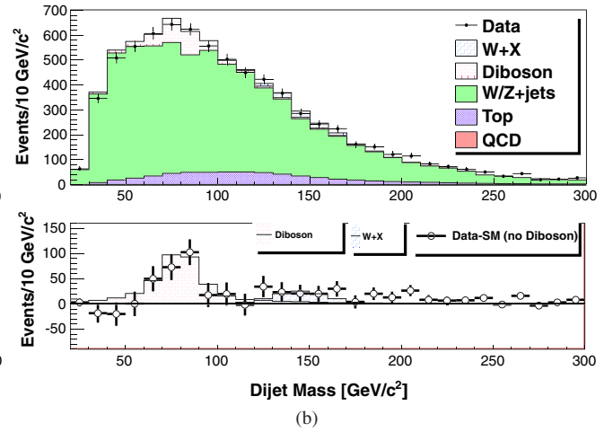
FIG. 11 (color online). Same distribution as in Fig. 10 shown separately for the electron (a) and muon (b) samples.
