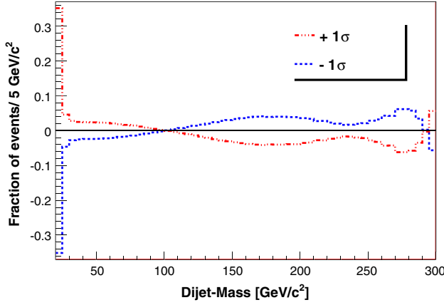
FIG. 2 (color online). Relative difference in the combined electron and muon samples between the nominal dijet-mass distribution and the one obtained by varying the jet-energy scale by \pm 1\sigma in W + \text{jets} events.
