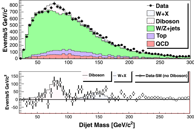
FIG. 10 (color online). Dijet mass distribution with fit results overlaid in the combined electron and muon data sets selected by applying an additional \Delta R(j_1, j_2) > 0.7 requirement and prior to incorporating the improvements discussed in the text. The bottom panel shows data with all fit background contributions subtracted except those from diboson production.
