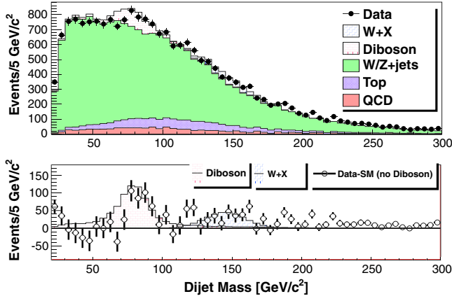
FIG. 7 (color online). Dijet mass distribution with fit results overlaid in the combined electron and muon data sets prior to incorporating the improvements discussed in the text, equivalent to updating the analysis described in Ref. [4] to the full CDF data set. The bottom panel shows data with all fit background contributions subtracted except those from diboson production.
