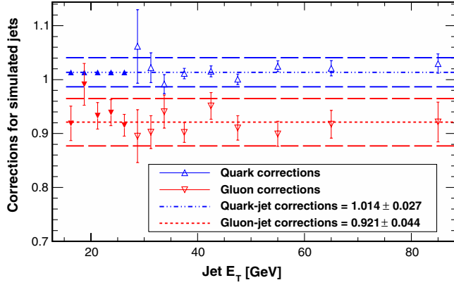
FIG. 1 (color online). Derived energy scale corrections for simulated quark jets and gluon jets as a function of jet E_T . The open triangles represent corrections derived jointly from the \gamma + jet and Z + jet balancing samples, while the filled triangles in the low-jet E_T region are obtained from the Z + jet sample only, assuming a constant correction for the quark-jet-energy scale. Error bars are from statistical sources only. The short-dashed lines show the fits to constant energy corrections, and the long-dashed lines represent the total systematic uncertainty bands on the correction determined by the fit.
