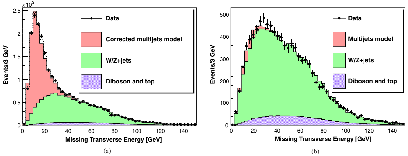
FIG. 6 (color online). Missing transverse-energy distribution for events containing electrons (a) and muons (b) from the selected sample. The distributions of observed data are shown with fit background overlaid.
