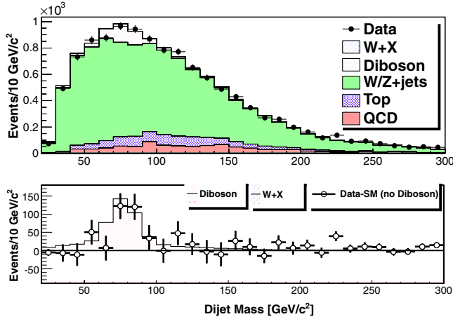
FIG. 13 (color online). Dijet mass distribution with fit results overlaid in the electron data set incorporating improved jet-energy-scale corrections for simulated quark and gluon jets and tunings on the multijet-background modeling. The bottom panel shows data with all fit background contributions subtracted except those from diboson production.
