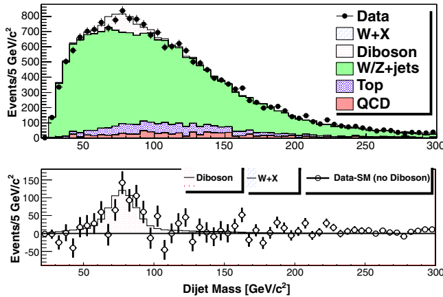
FIG. 14 (color online). Dijet mass distribution with fit results overlaid in the combined electron and muon data sets incorporating improved jet-energy-scale corrections for simulated quark and gluon jets and tunings on the multijet-background modeling. The bottom panel shows data with all fit background contributions subtracted except those from diboson production.
