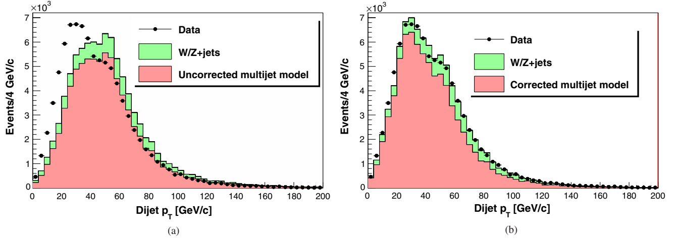
FIG. 4 (color online). Transverse-momentum distribution of the two-jet system in the multijet-enriched control sample as observed in the data (circles) and as predicted by the W/Z + \text{jets} simulation (light shaded histogram) and the nonelectron-based model (dark shaded histogram) before (a) and after (b) application of tunings to the nonelectron-based multijet model. The magnitude of W/Z + \text{jets} contributions is normalized to the NLO calculations [23], while the magnitude of the multijet model is obtained from the data.
