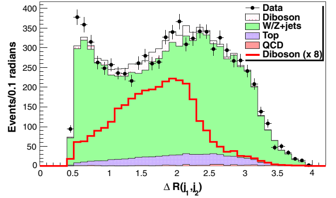
FIG. 9 (color online). \Delta R(j_1, j_2) distribution in the muon sample as observed in the data and as predicted by the models incorporating improved jet-energy-scale corrections for simulated quark and gluon jets. The diboson distribution (red line) magnified by a factor of 8 is also shown as an example of the \Delta R(j_1, j_2) distribution for a heavy-particle decay.
