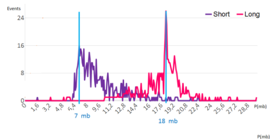
Figure 8. Increase vacuum after the initial vacuum stage
