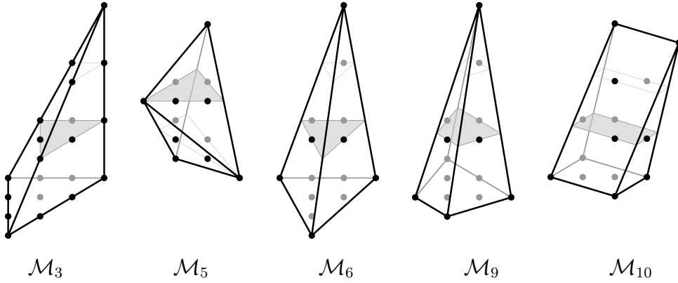
Figure 2.10: The five hollow 3-polytopes of width three. This picture has been taken from Averkov et al [AKW15].
