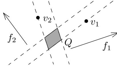
Figure 1.11: A boxed polygon. Q is the parallelepiped f_1^{-1}([0, 1]) \cap f_2^{-1}([0, 1]) .
