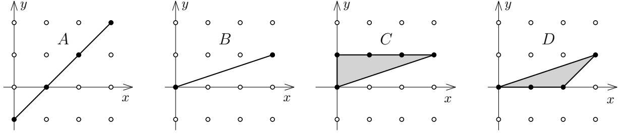
Figure 2.4: Polytopes A, B, C, D \subset \mathbb{R}^2 are lifts of [0, 3] \subset \mathbb{R} under projection \pi(x, y) = x . A and B are tight lifts; C and D are not.
