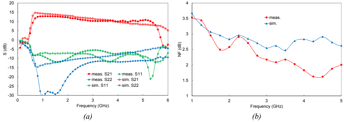
Fig. 10. (a) Measured and simulated Scattering parameters versus frequency for the DA with resistive line terminations, (b) measured and simulated noise figure (NF) versus frequency.
