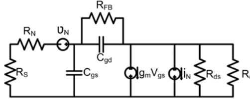
Fig. 2. Small signal model for noise temperature analysis in a HEMT.
