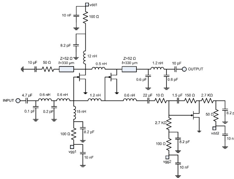
Fig. 9. Schematic of DA with active gate line termination.
