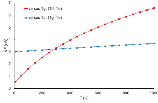
Fig. 1. Noise figure of a distributed amplifier in (9) and (11) versus line termination temperature.
