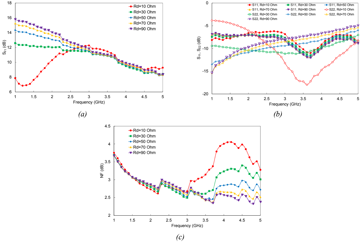
Fig. 6. Simulated Scattering parameters versus frequency and drain load for the distributed amplifier with resistive line terminations. Gate load 50 \Omega . (a) S_{21} ; (b) S_{11} and S_{22} . (c) Simulated noise figure versus frequency and drain load for the distributed amplifier with resistive line terminations.
