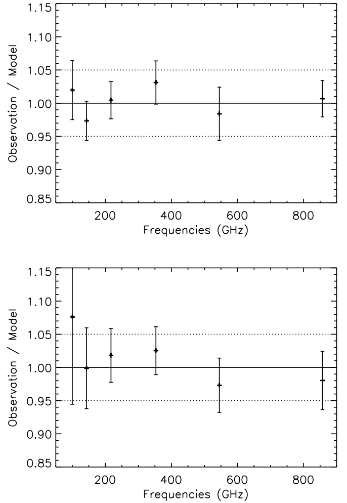
Fig. 9. Ratio of the flux densities measured by HFI and computed from the ESA2 (Uranus, top ) and ESA3 (Neptune, bottom ) models from Moreno (2010). At 545 and 857 GHz, the measurements are not independent measurements of the planet flux densities, since the 545 and 857 GHz channels have been re-calibrated to match the average of the Uranus and Neptune flux density given by the models.
