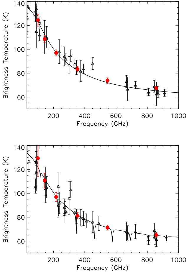
Fig. 10. Variation of brightness temperature with frequency for Uranus ( top ) and Neptune ( bottom ). The brightness temperatures derived from the flux densities measured using aperture photometry on HFI maps are the red points. The continuous lines are the ESA2 (Uranus) and ESA3 (Neptune) models from Moreno (2010) . The scale of the models is known at about the 5% level, and the relative inter-frequency uncertainty is expected to be of the order of 2%. At 545 and 857 GHz, the measurements are not independent determinations of the planet flux densities, since the 545 and 857 GHz channels have been re-calibrated to match the average of the Uranus and Neptune flux density given by the models. The other data points are extracted from the literature.
