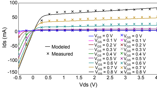
Fig. 2 Comparison of I/V measured and modeled characteristics.
