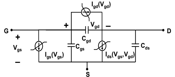
Fig. 1 Electrical equivalent circuit of the extracted model.
